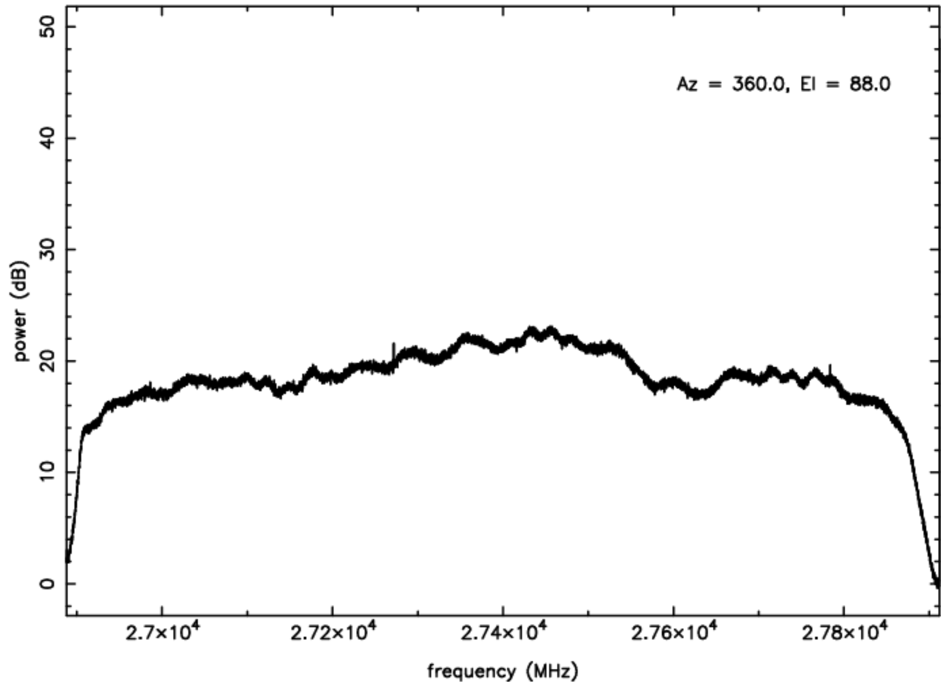
Ka-band RFI plot (mean power) – IF B – ea14
