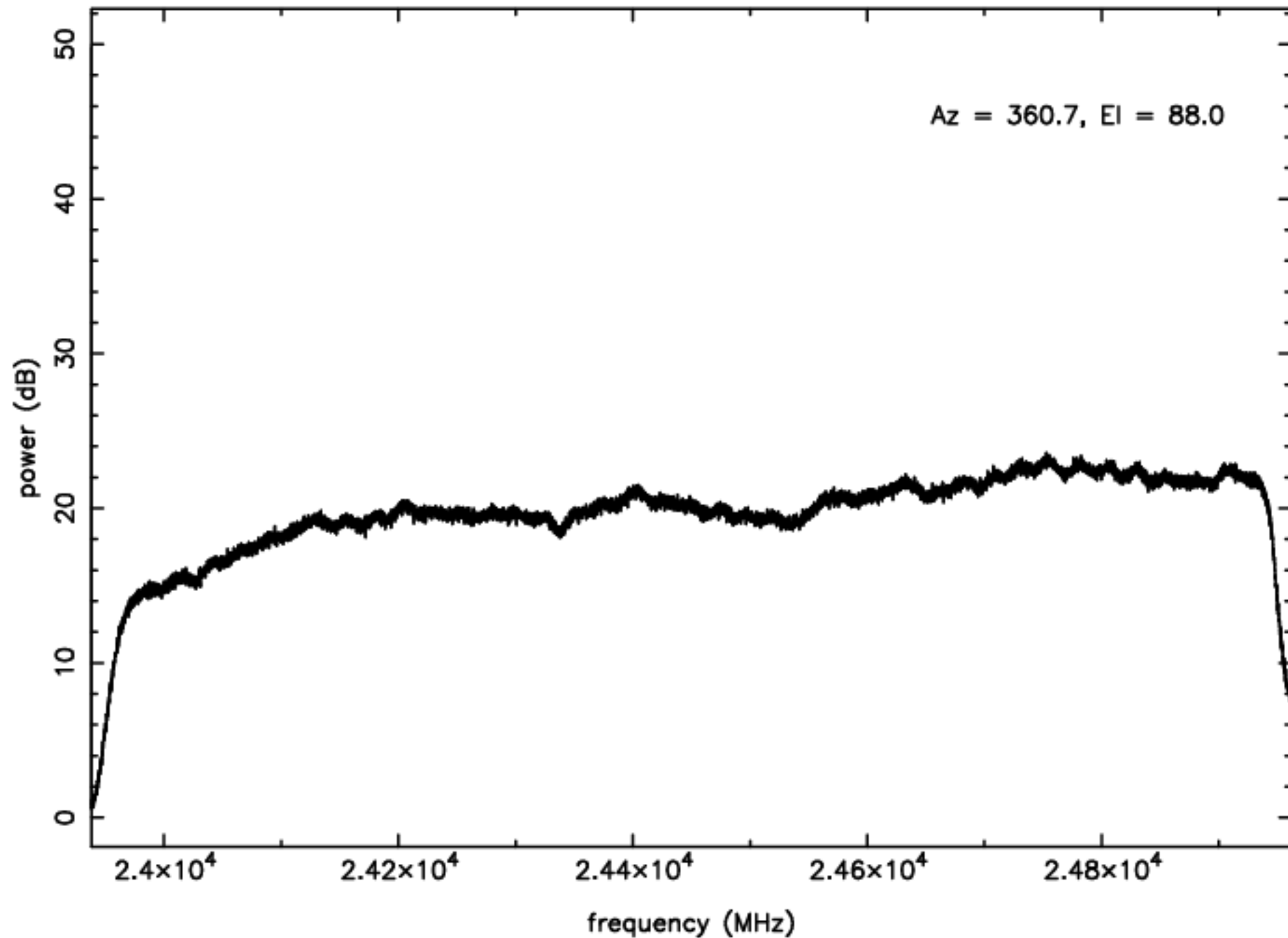
K-band RFI plot (mean power) – IF D – ea14
