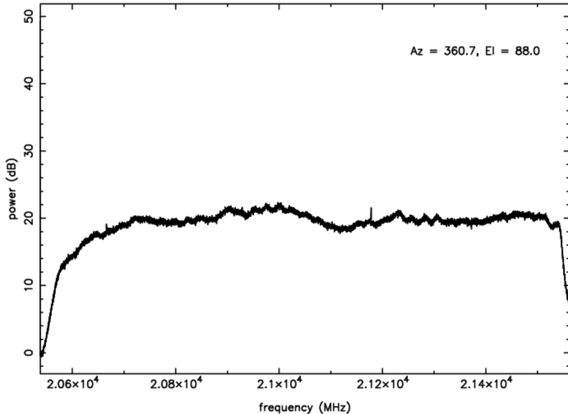
K-band RFI plot (mean power) – IF B – ea14
