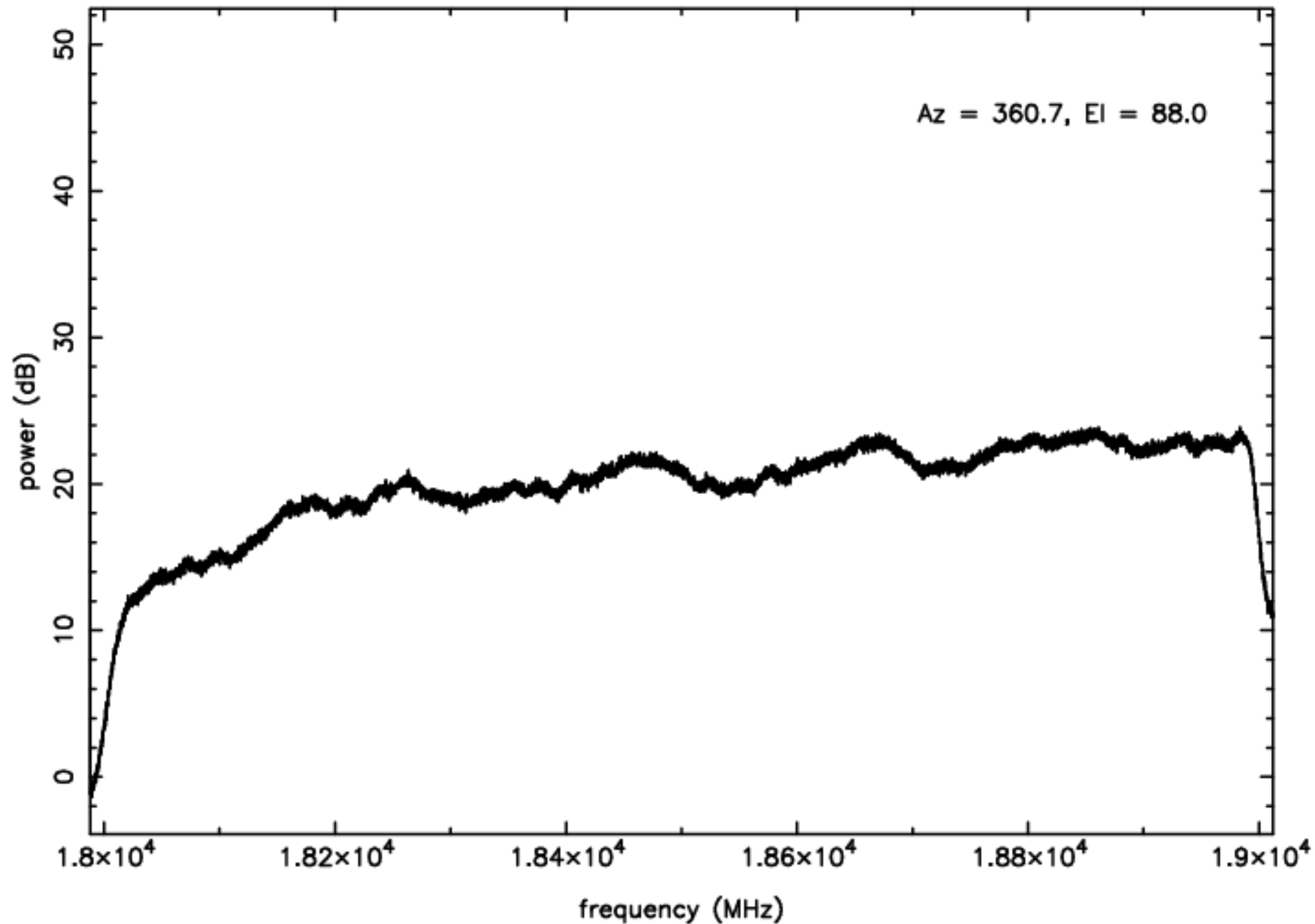
K-band RFI plot (mean power) – IF D – ea14
