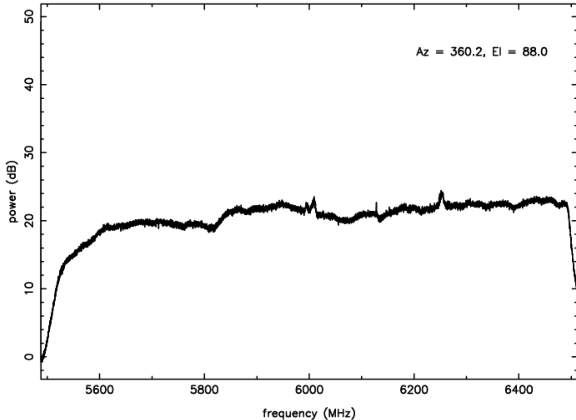
C-band RFI plot (mean power) – IF B – ea14
