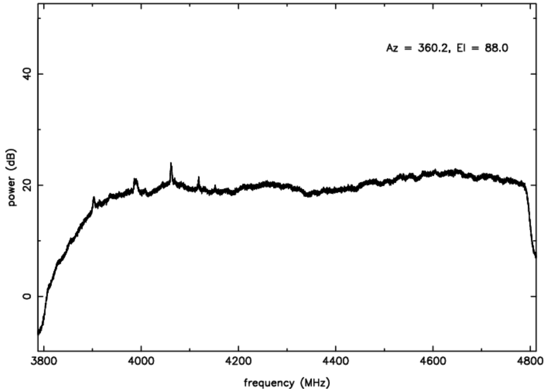
C-band RFI plot (mean power) – IF D – ea14
