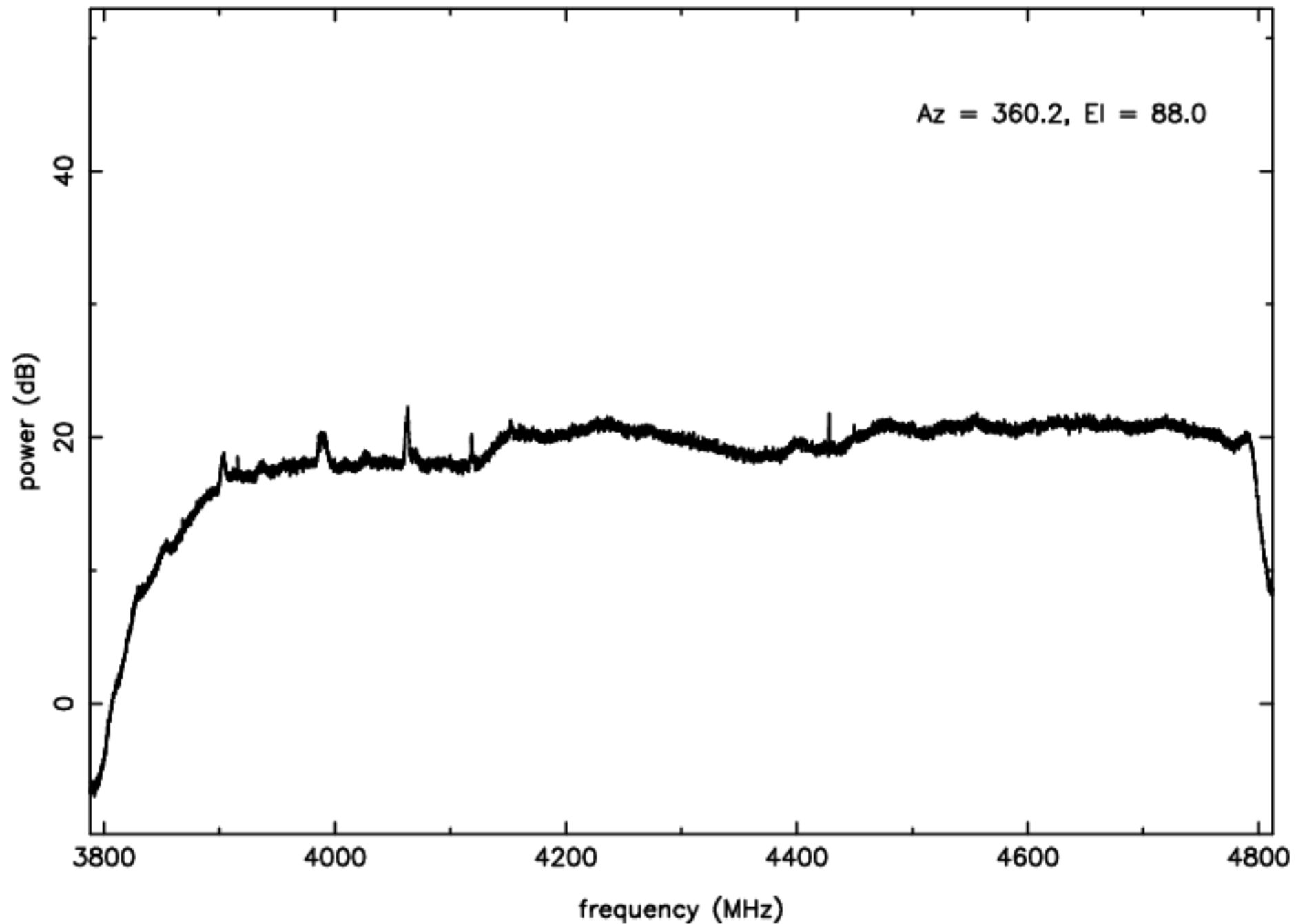
C-band RFI plot (mean power) – IF B – ea14
