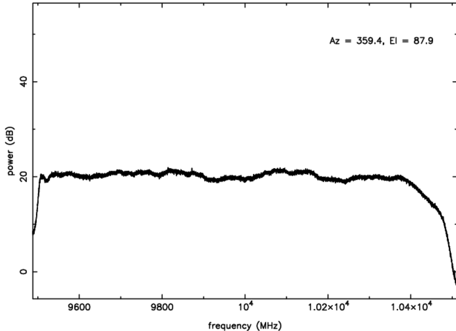
X-band RFI plot (mean power) – IF B – ea07
