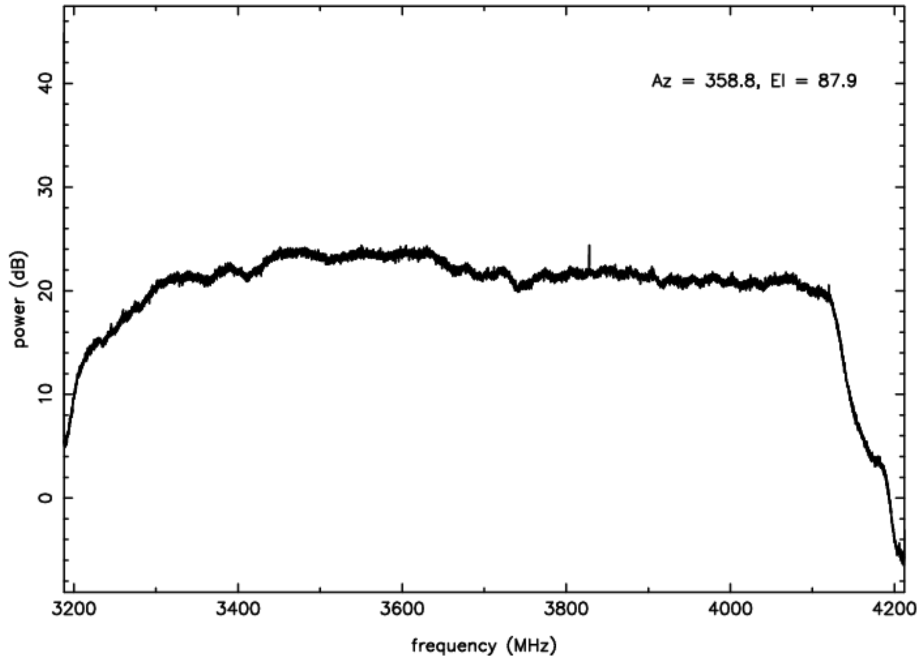
S-band RFI plot (mean power) – IF D – ea07
