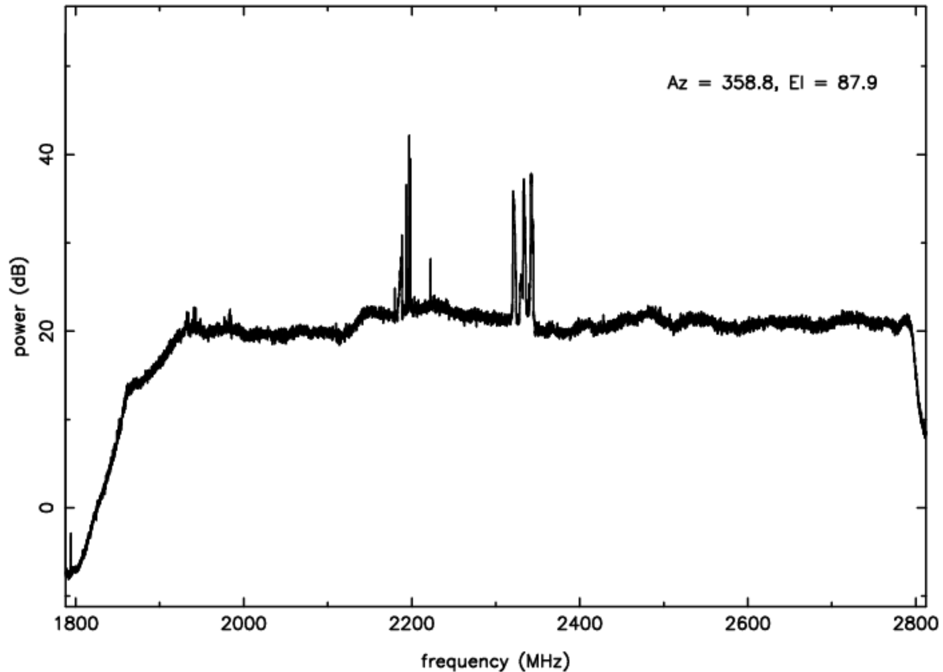
S-band RFI plot (mean power) – IF B – ea07
