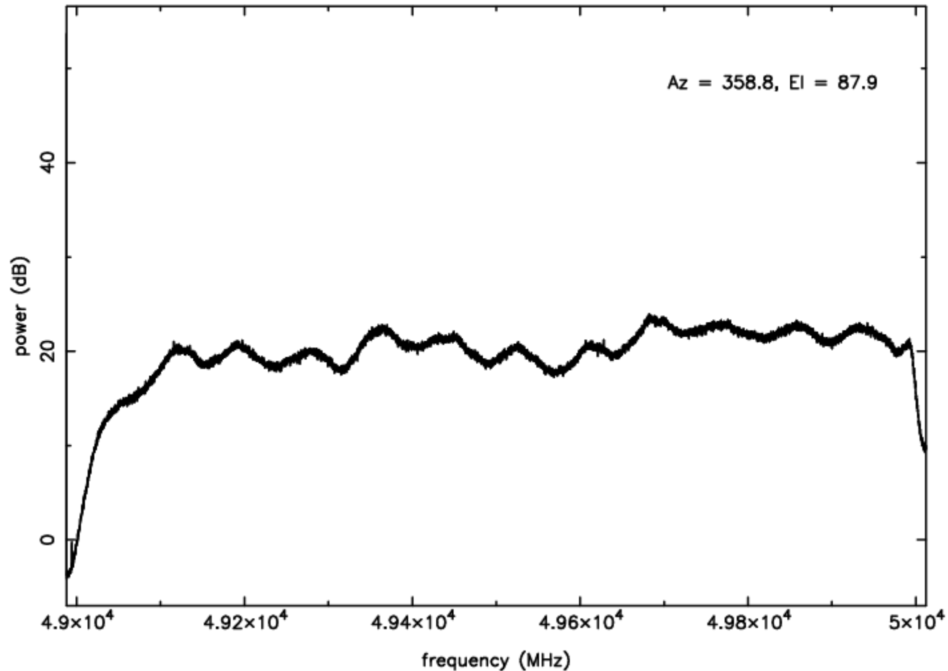
Q-band RFI plot (mean power) – IF B – ea07
