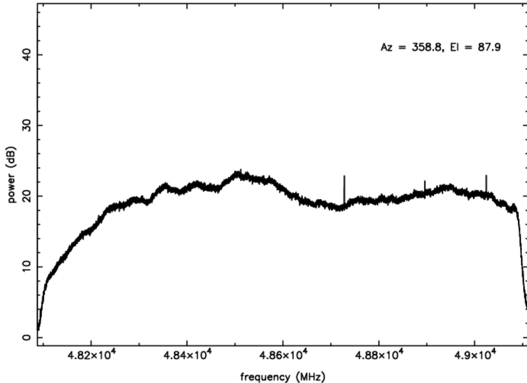
Q-band RFI plot (mean power) – IF D – ea07
