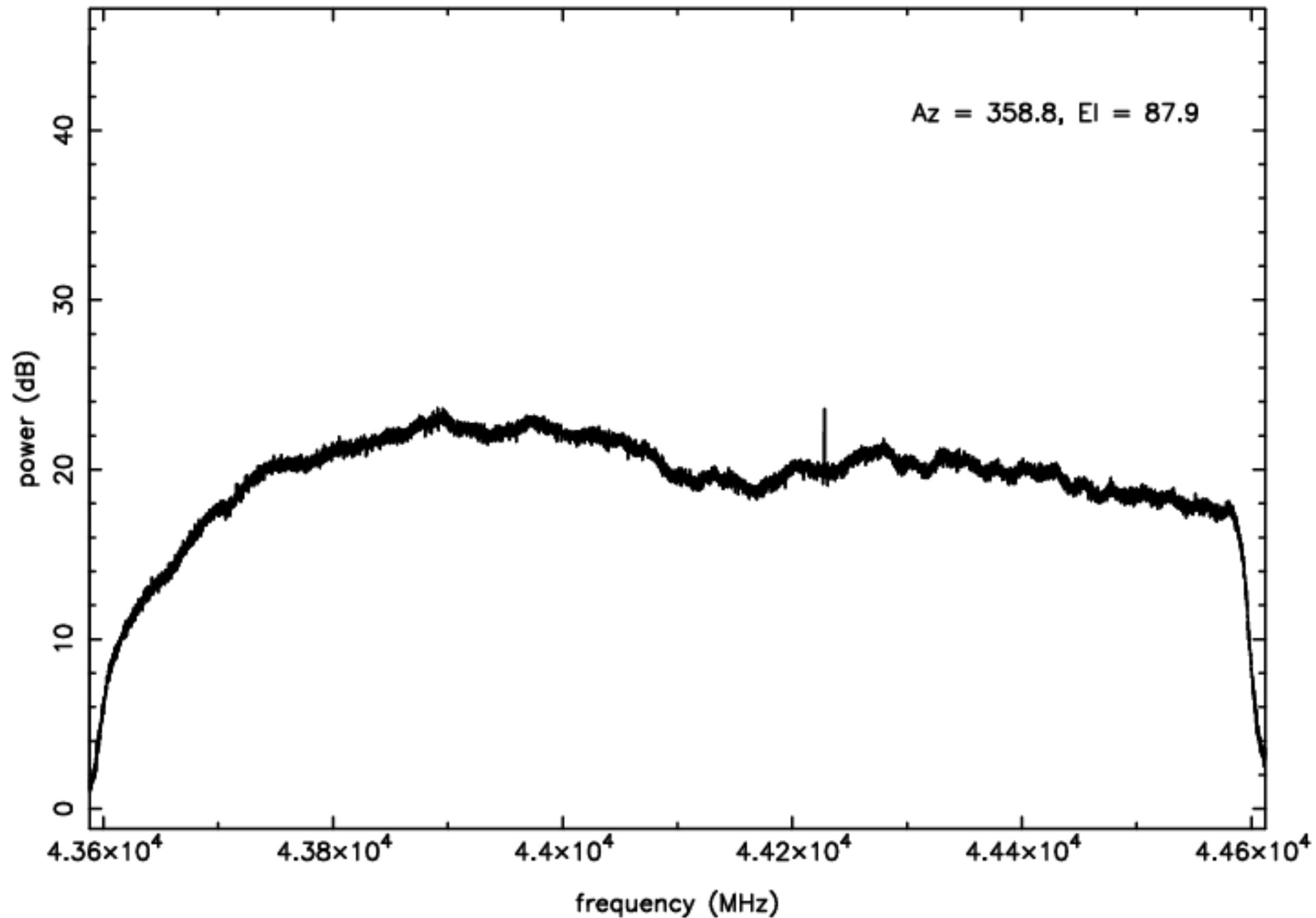
Q-band RFI plot (mean power) – IF D – ea07
