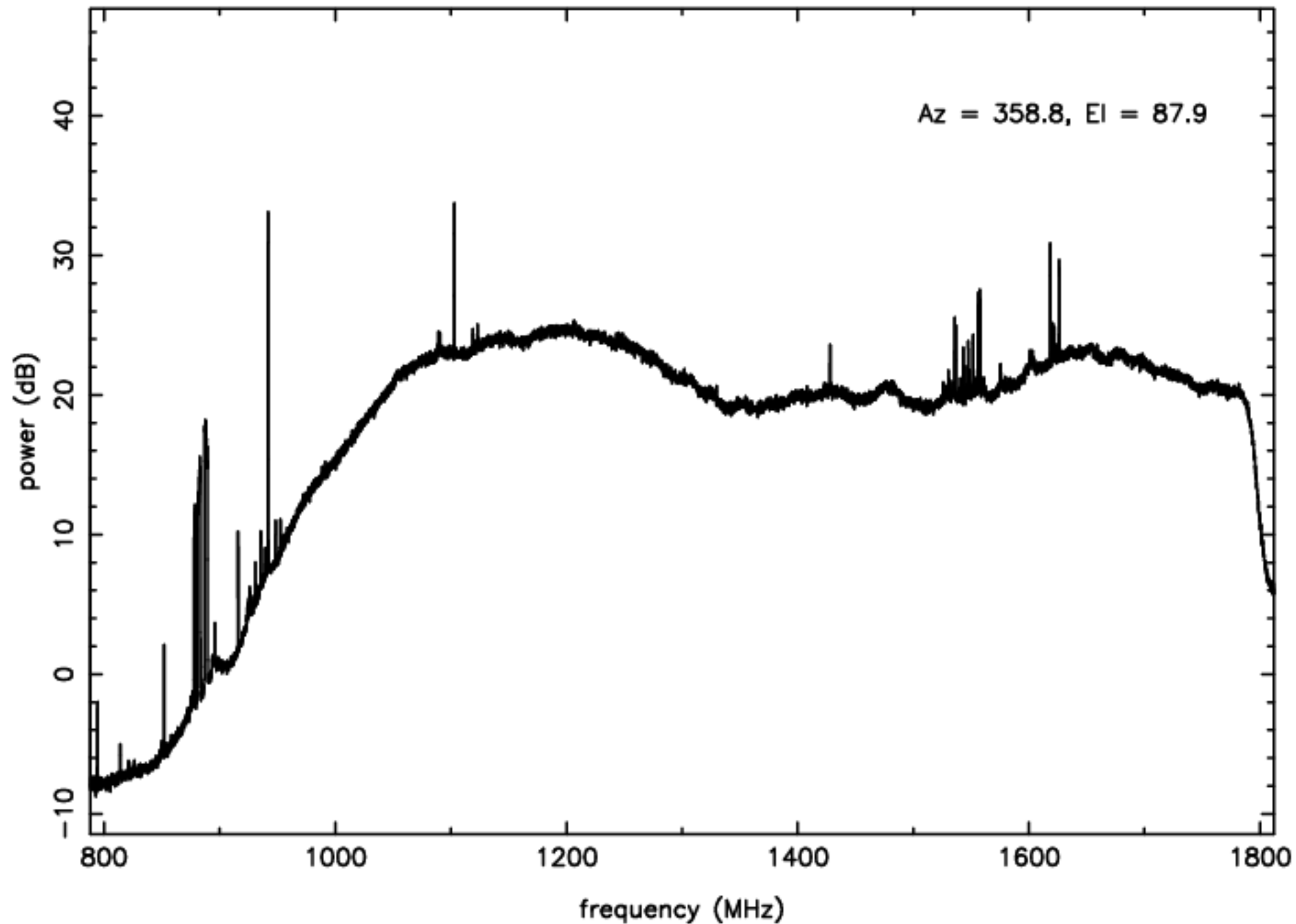
L-band RFI plot (mean power) – IF D – ea07
