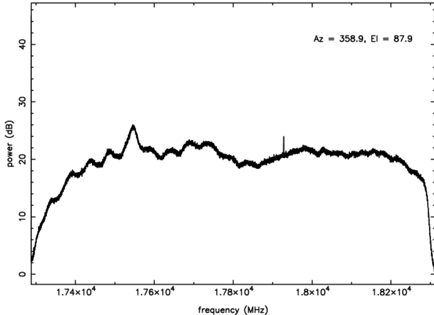
Ku-band RFI plot (mean power) – IF D – ea07
