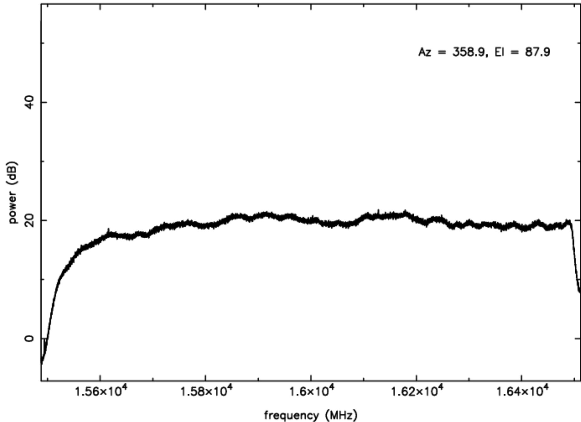
Ku-band RFI plot (mean power) – IF B – ea07
