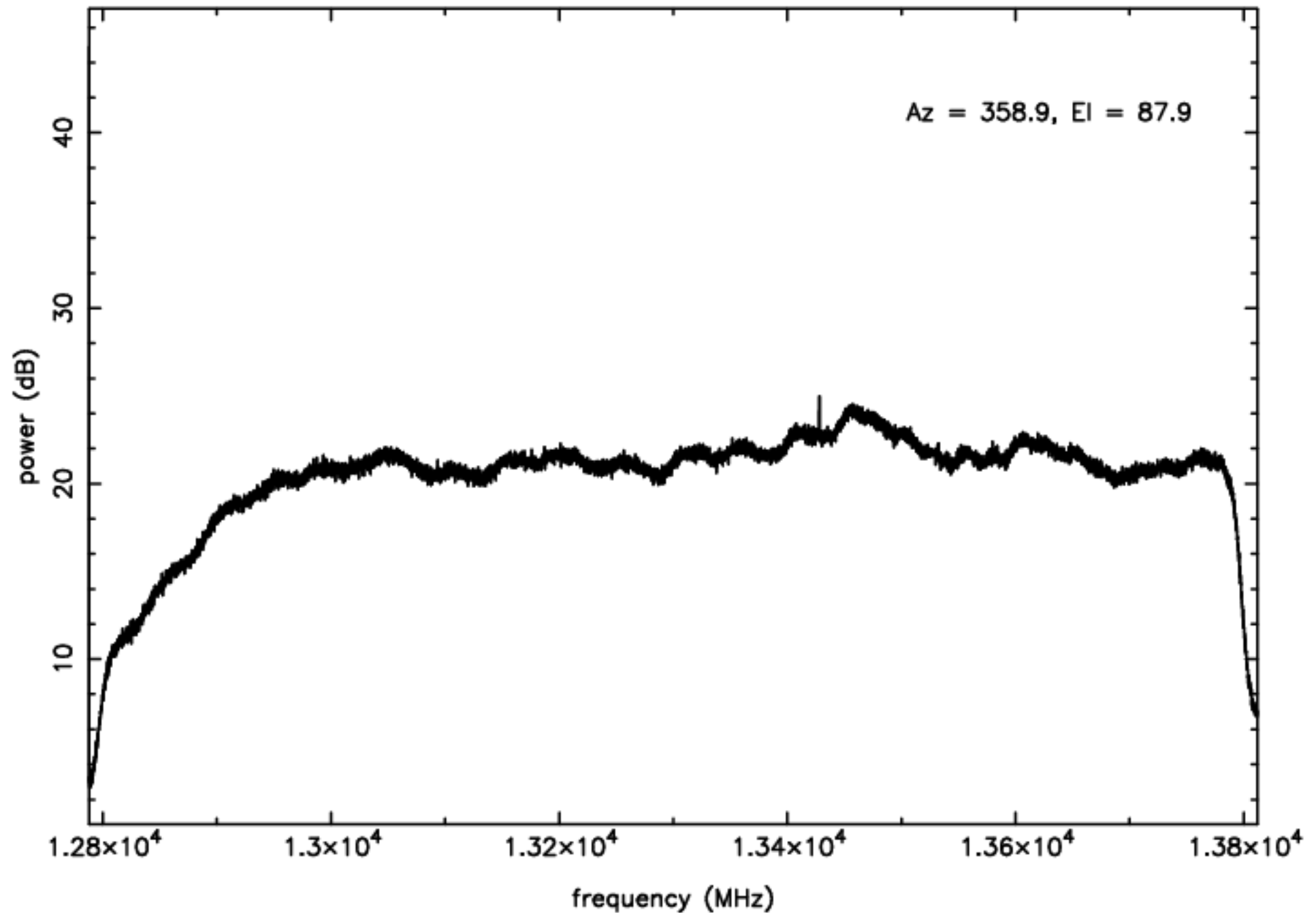
Ku-band RFI plot (mean power) – IF D – ea07
