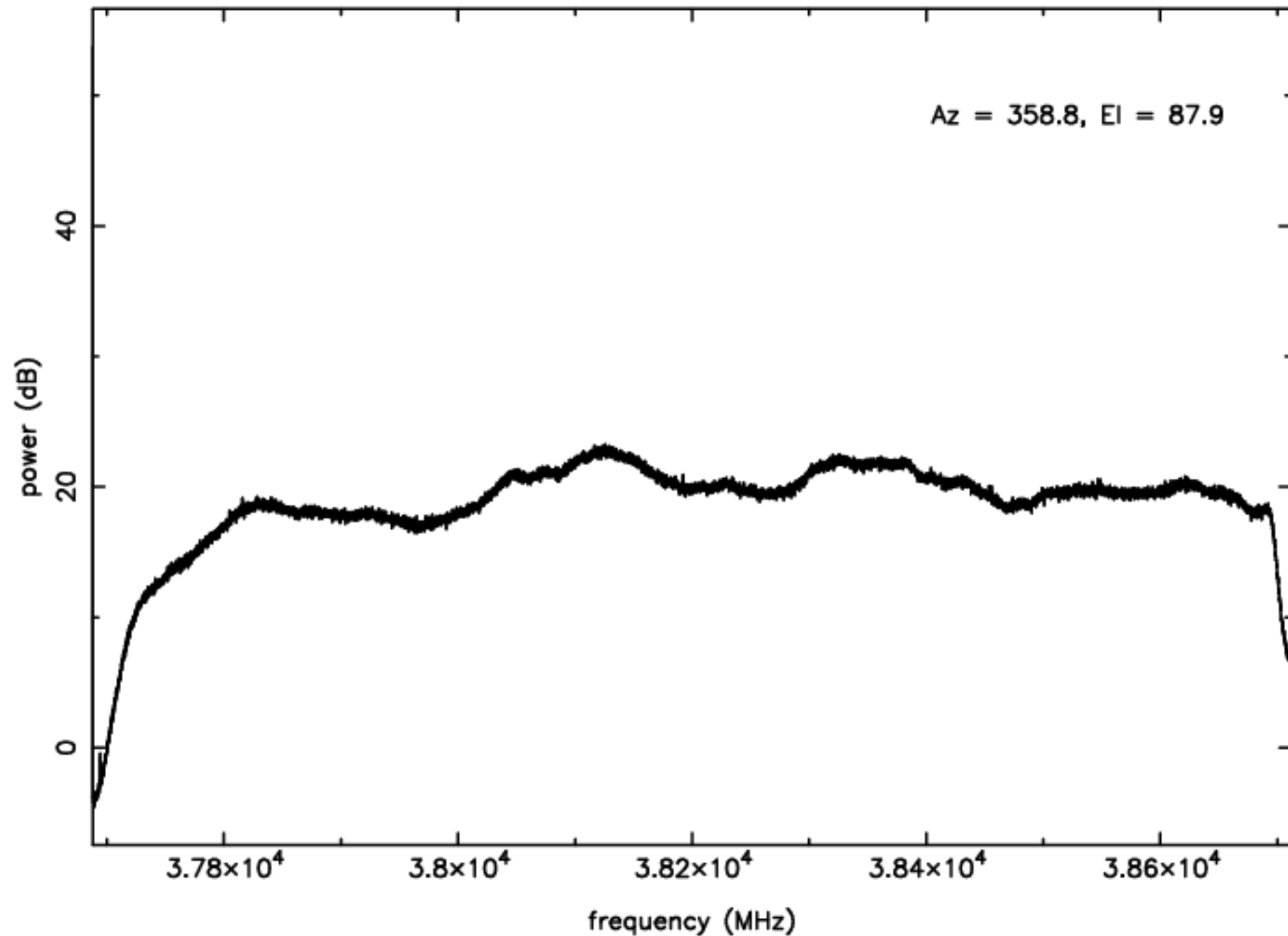
Ka-band RFI plot (mean power) – IF B – ea07
