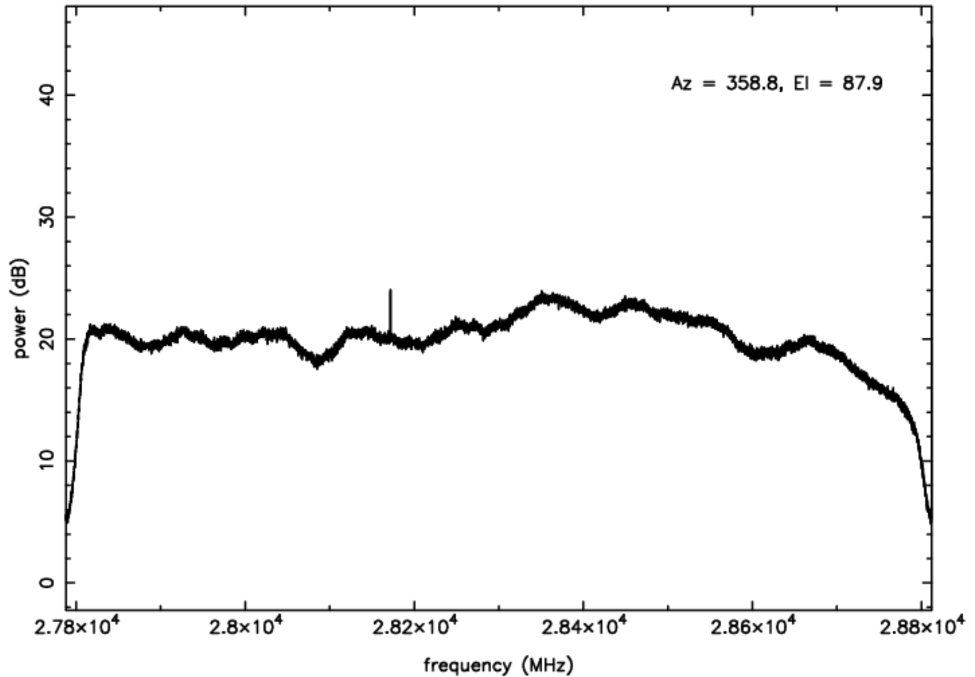
Ka-band RFI plot (mean power) - IF D - ea07
