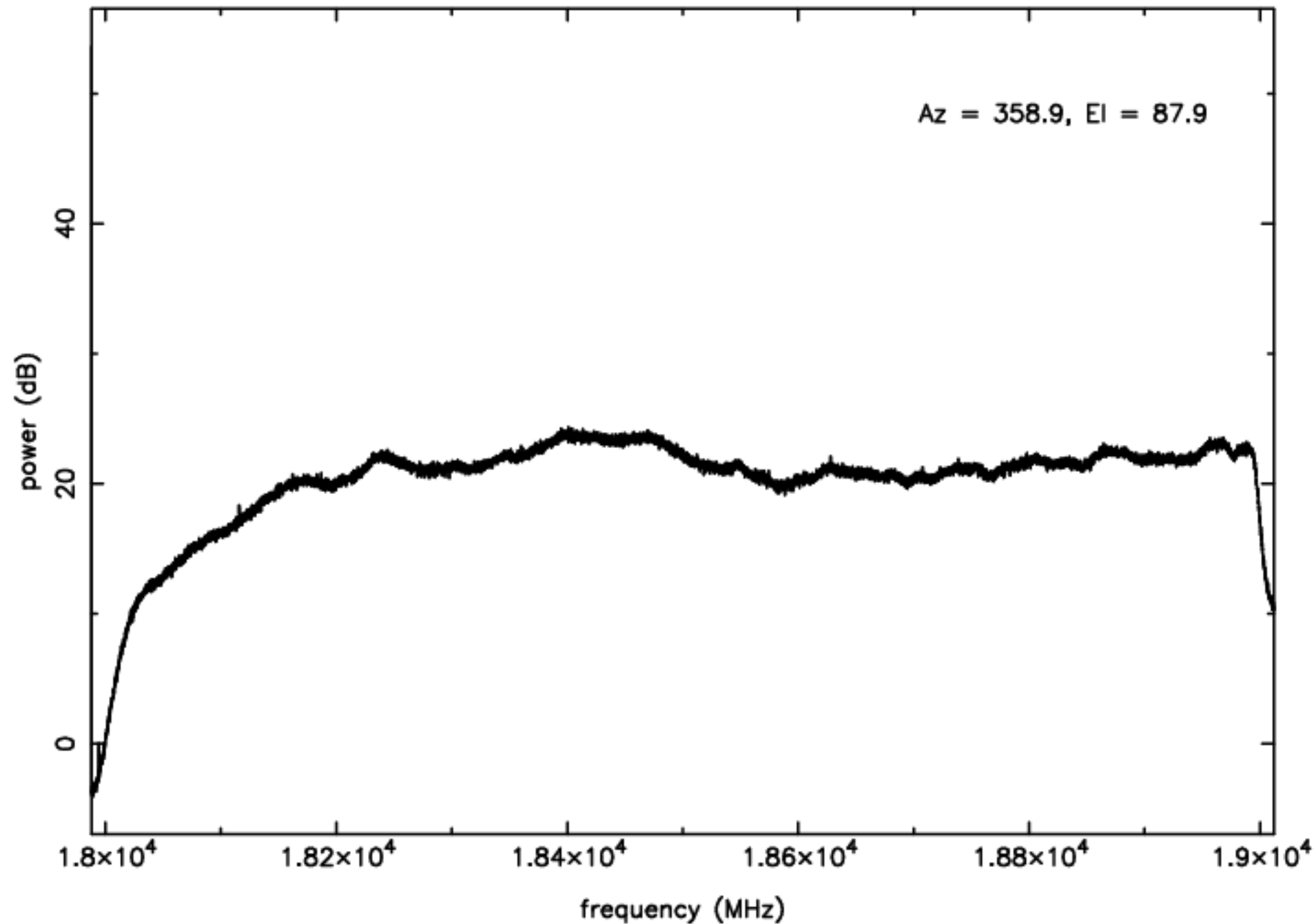
K-band RFI plot (mean power) – IF B – ea07
