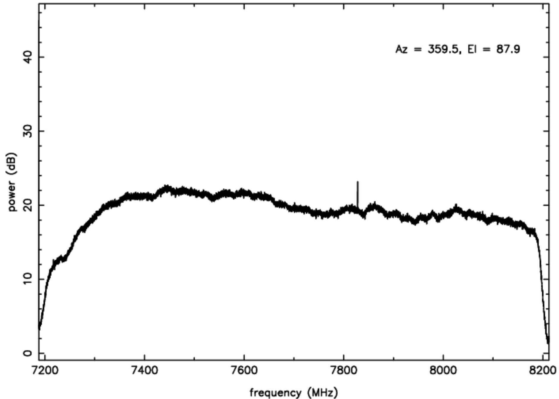
C-band RFI plot (mean power) – IF D – ea07
