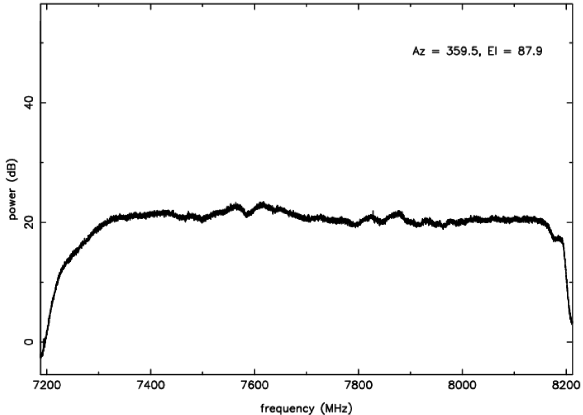
C-band RFI plot (mean power) – IF B – ea07
