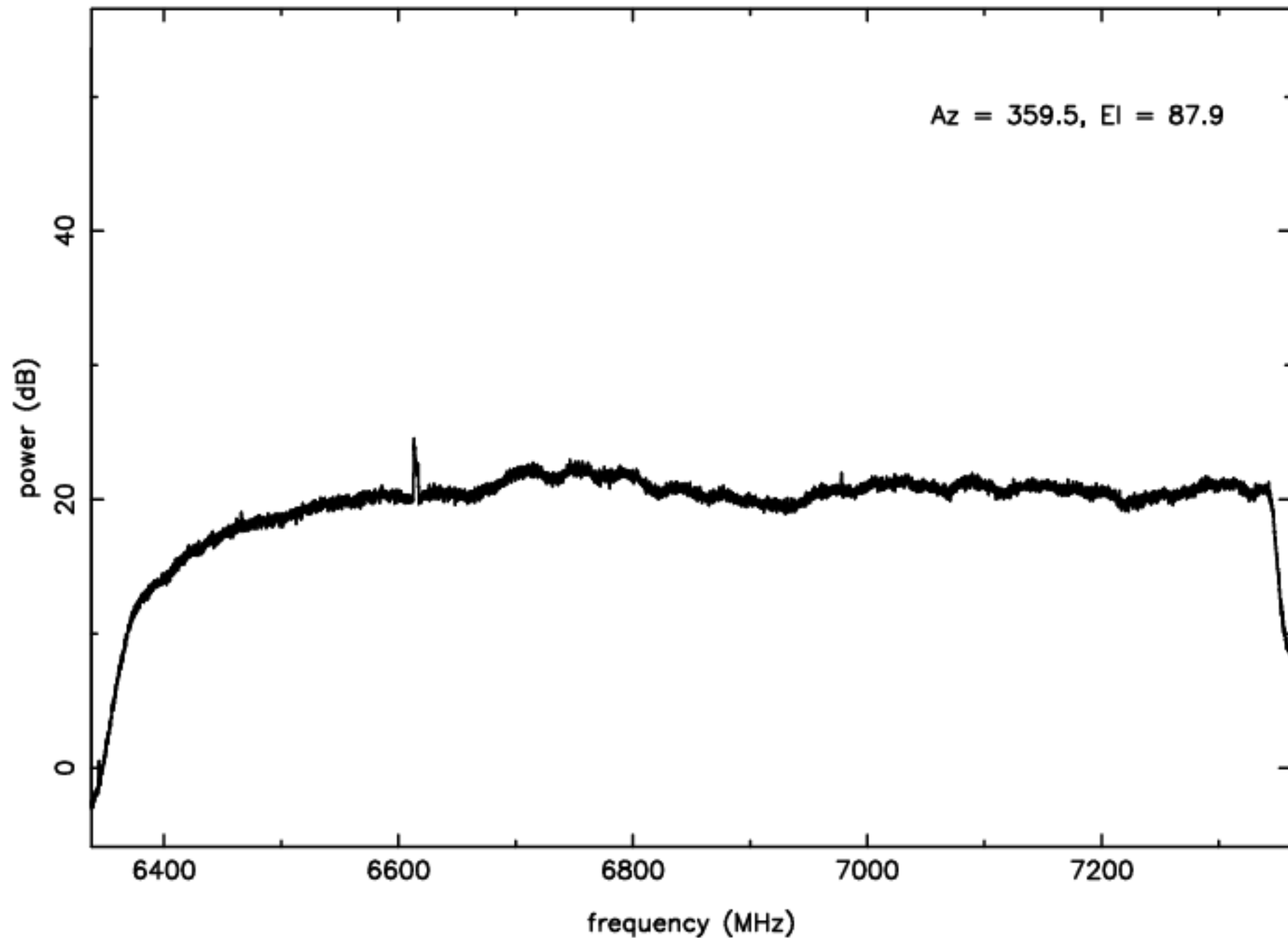
C-band RFI plot (mean power) – IF B – ea07
