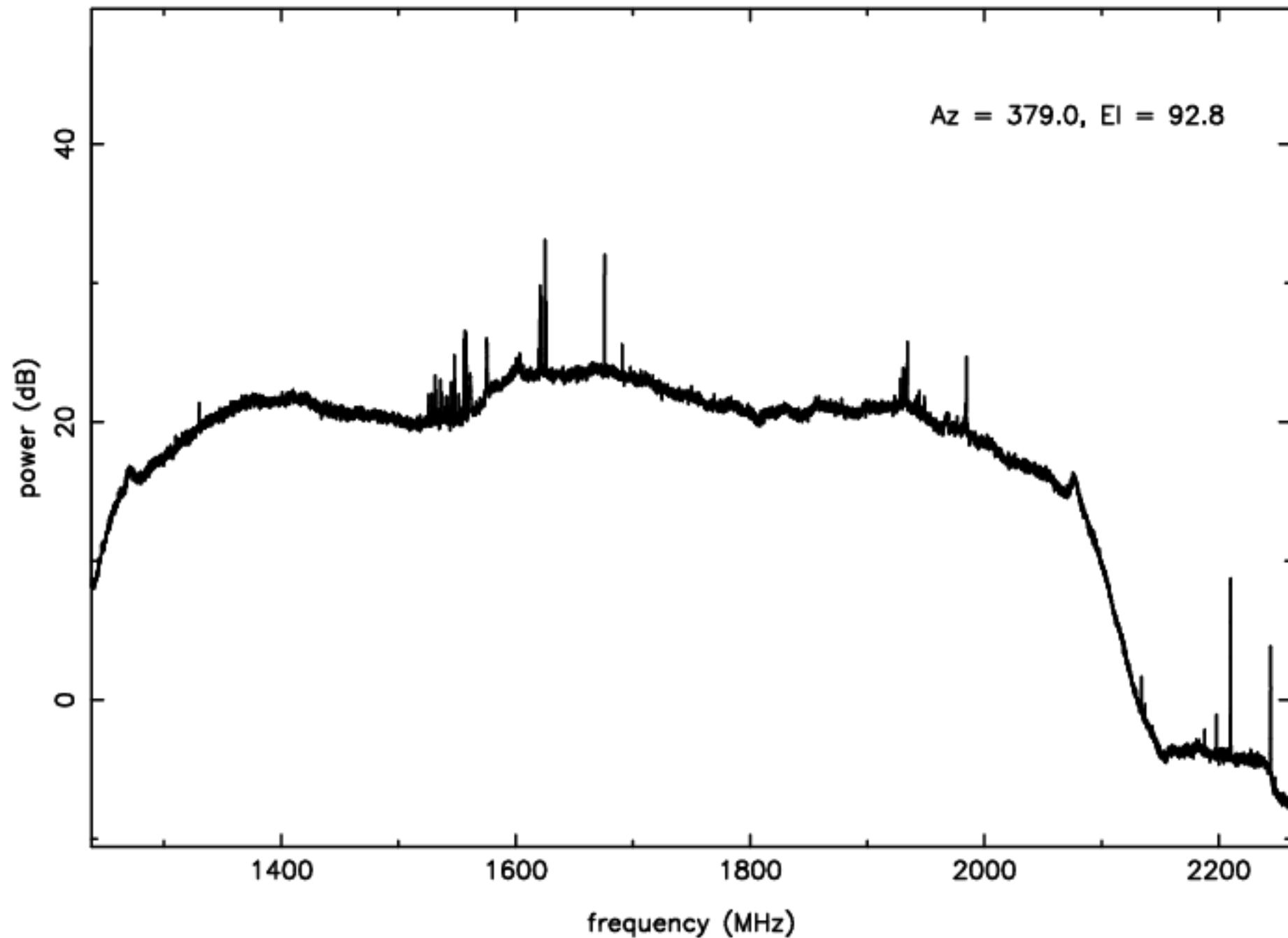
L-band RFI plot (mean power) – IF D – ea10
