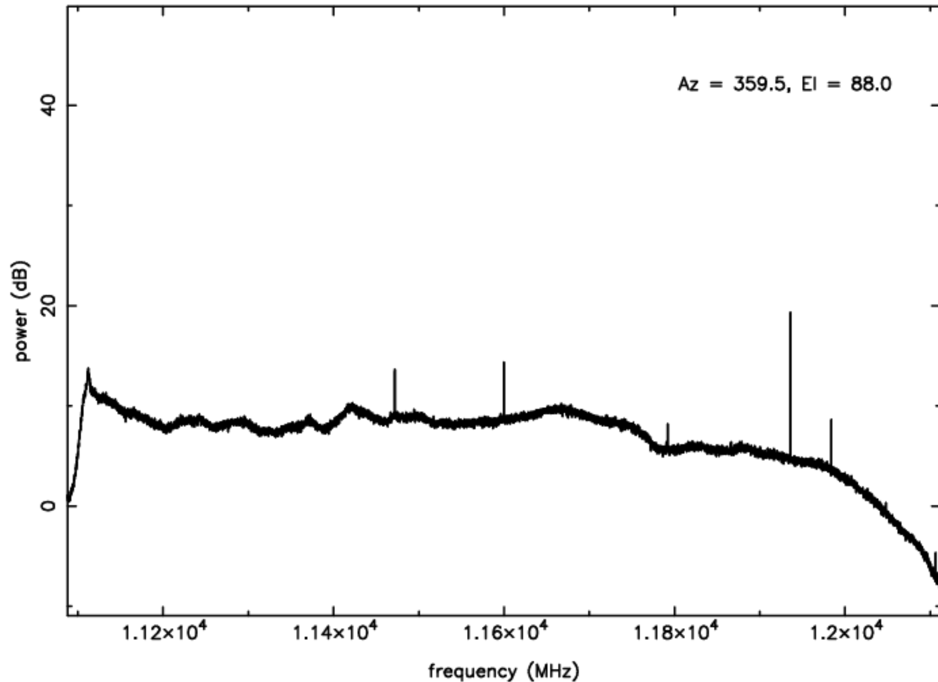
X-band RFI plot (mean power) – IF D – ea10
