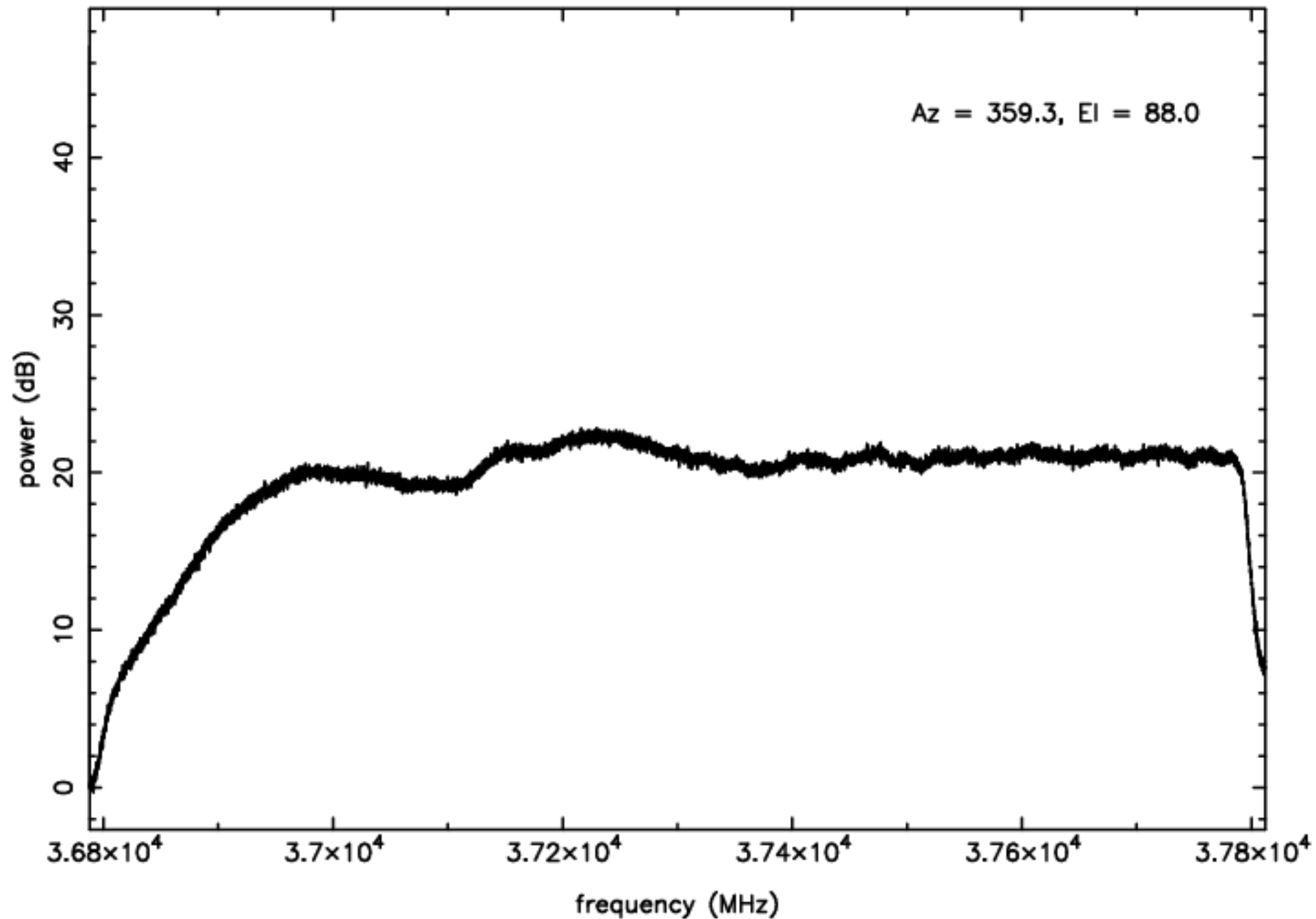
Ka-band RFI plot (mean power) – IF D – ea10
