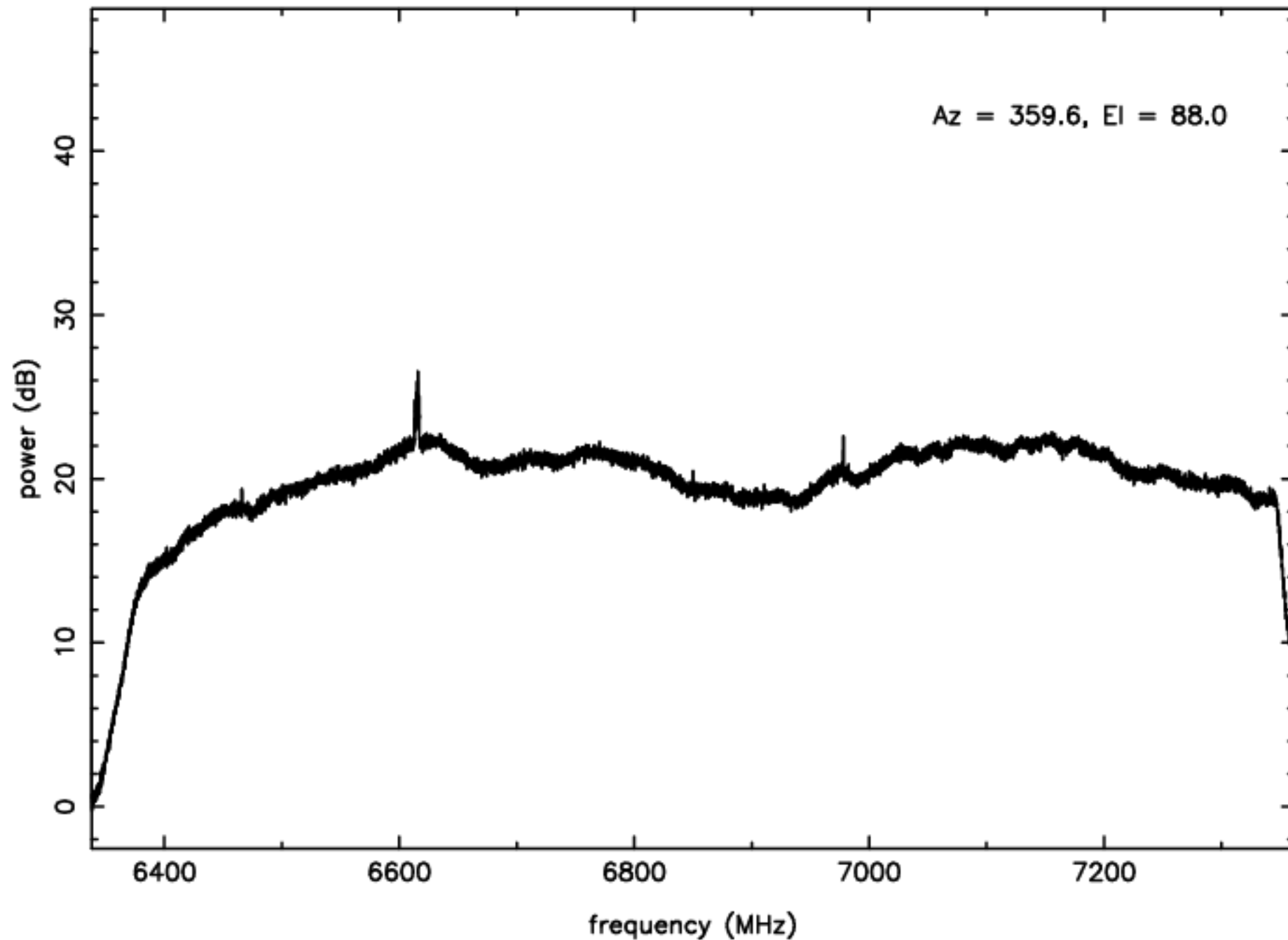
C-band RFI plot (mean power) – IF B – ea10
