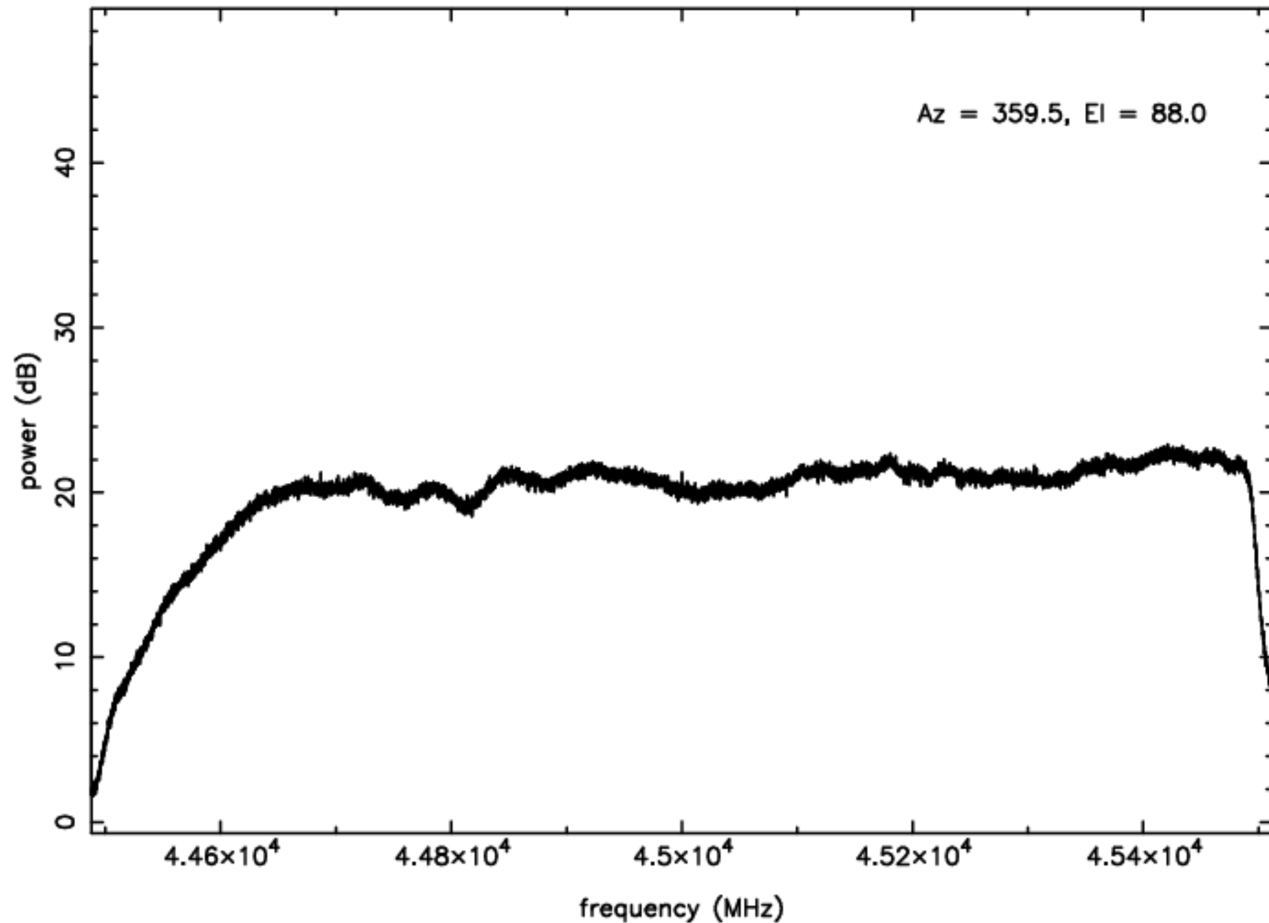
Q-band RFI plot (mean power) – IF D – ea10
