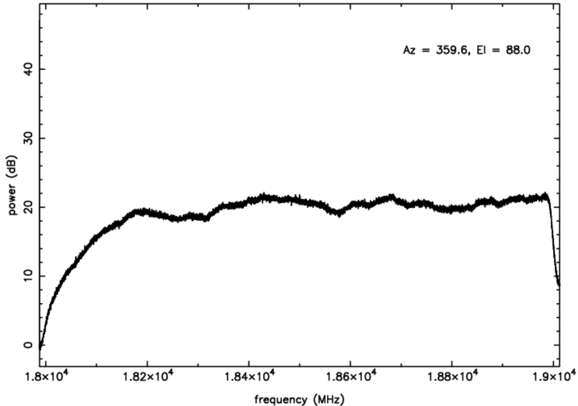
K-band RFI plot (mean power) – IF D – ea10
