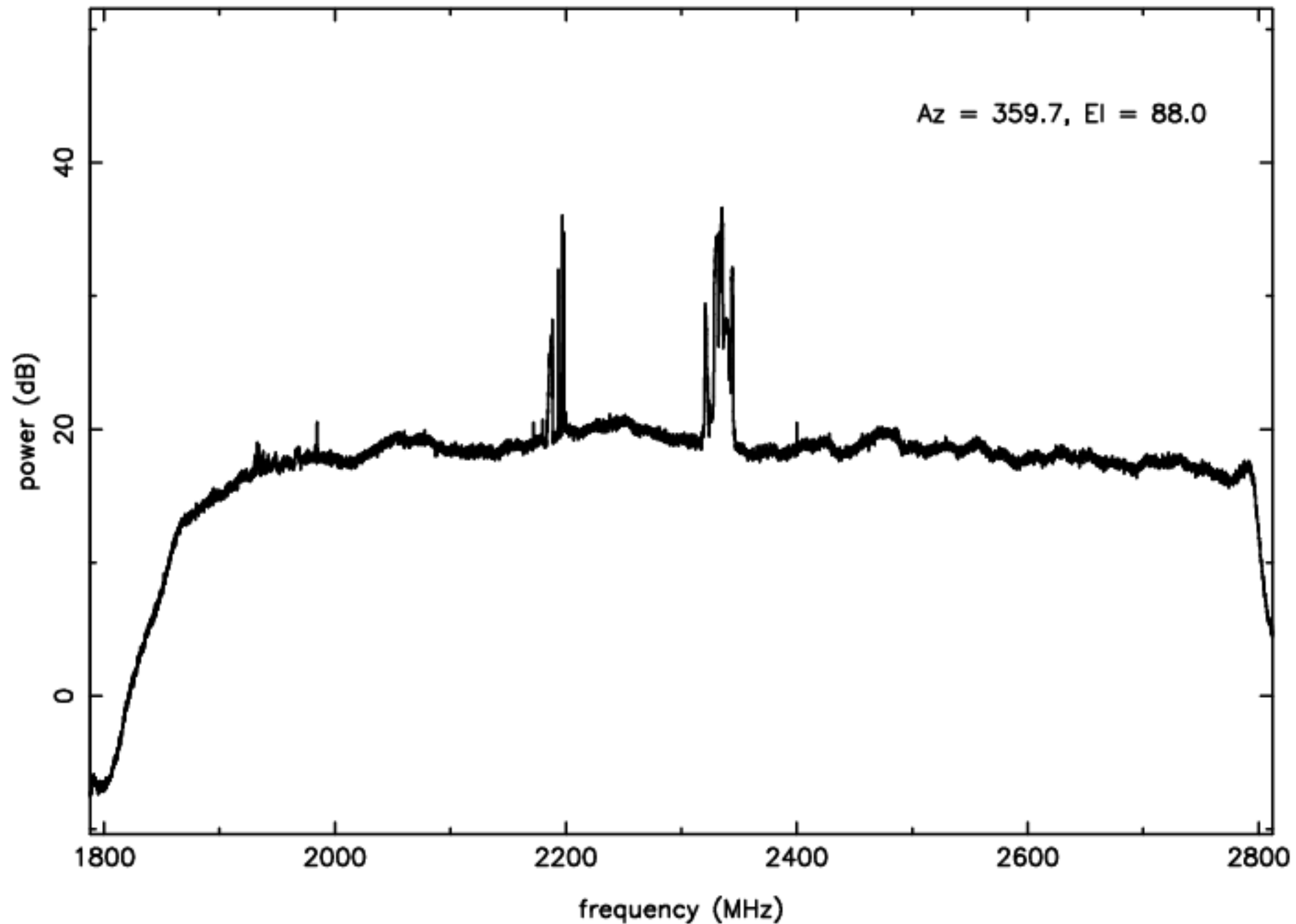
S-band RFI plot (mean power) – IF B – ea24
