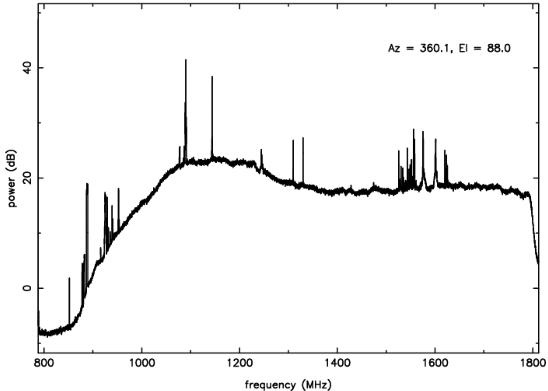
L-band RFI plot (mean power) – IF B – ea24
