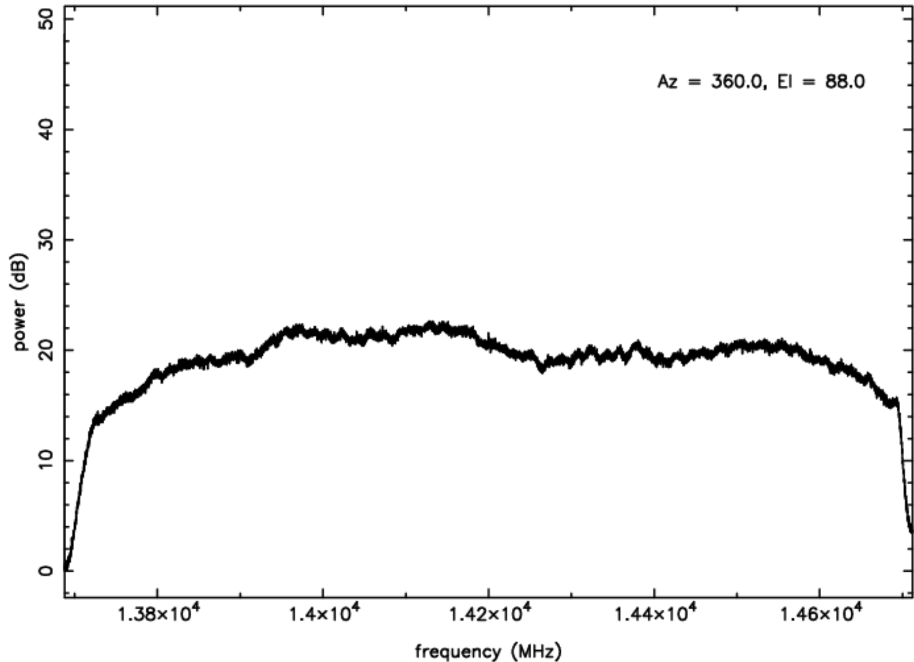
Ku-band RFI plot (mean power) - IF B - ea24
