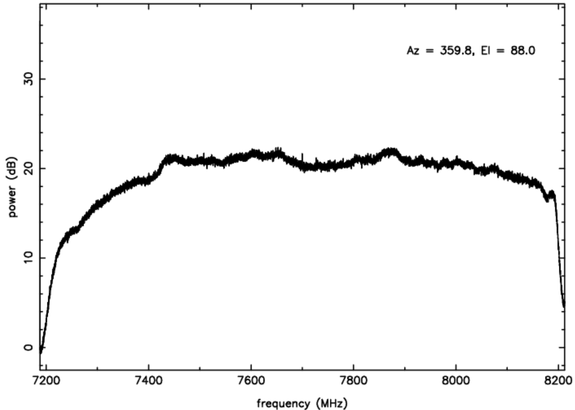
C-band RFI plot (mean power) – IF D – ea24
