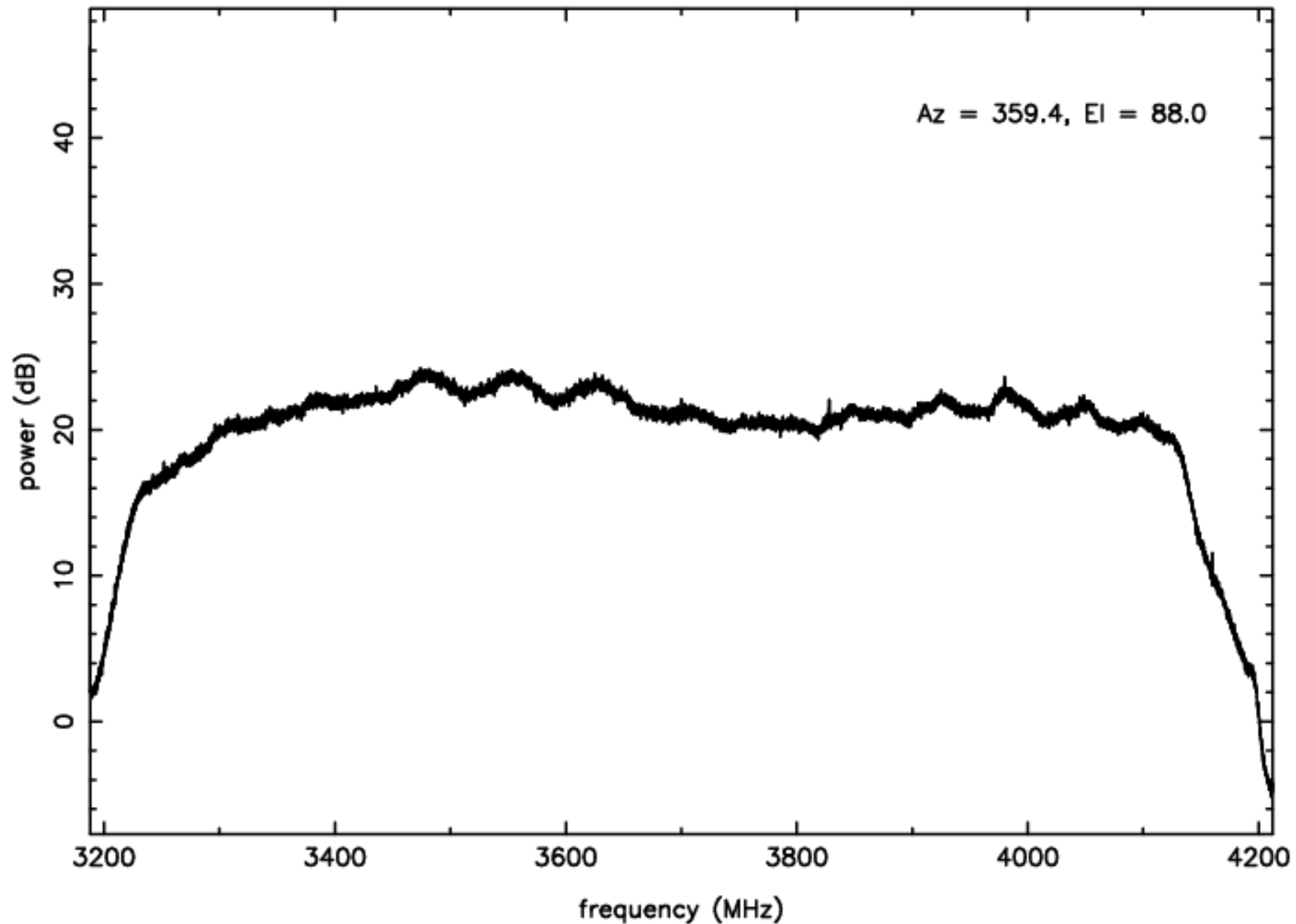
S-band RFI plot (mean power) – IF B – ea10
