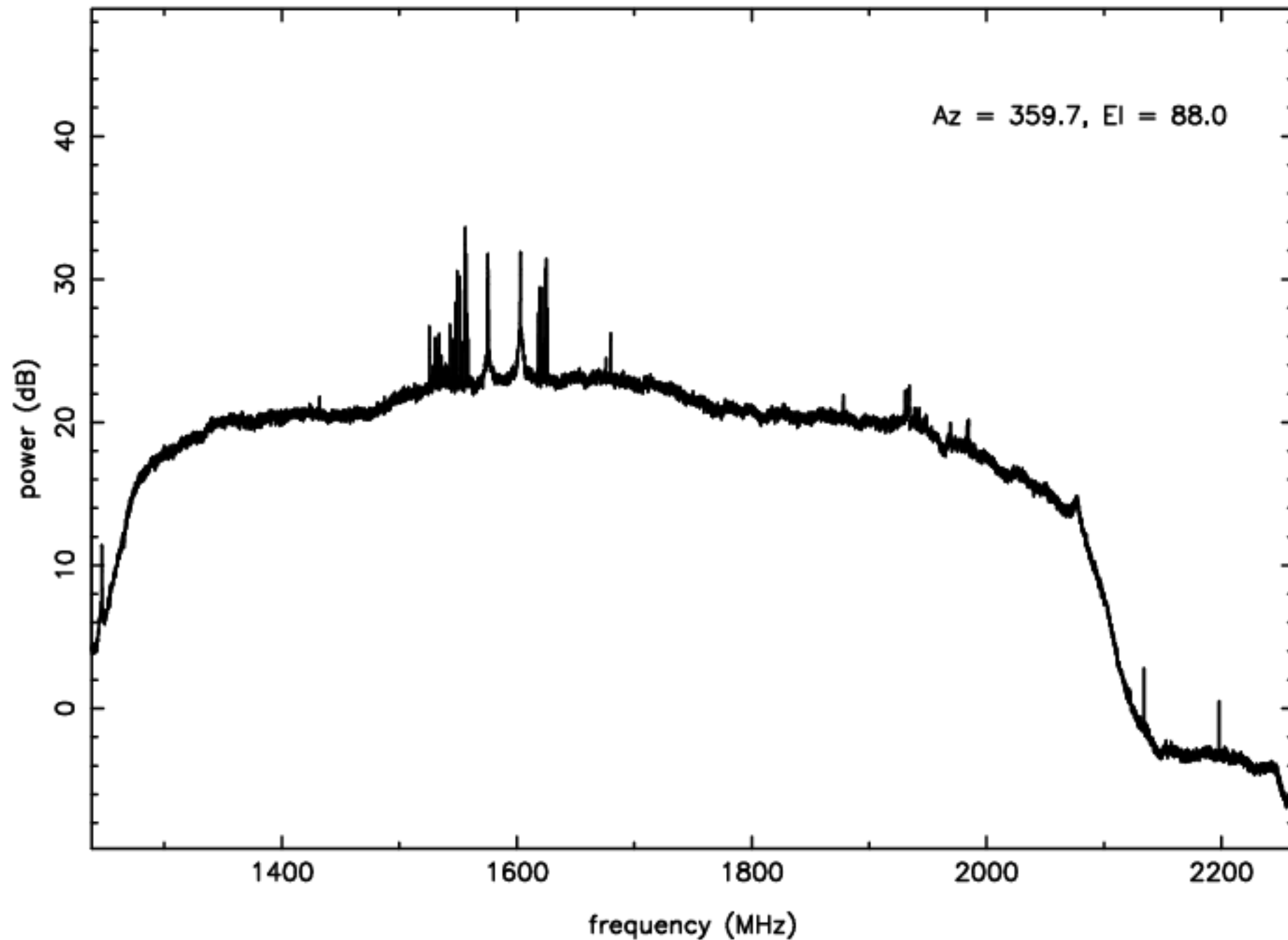
L-band RFI plot (mean power) – IF B – ea10
