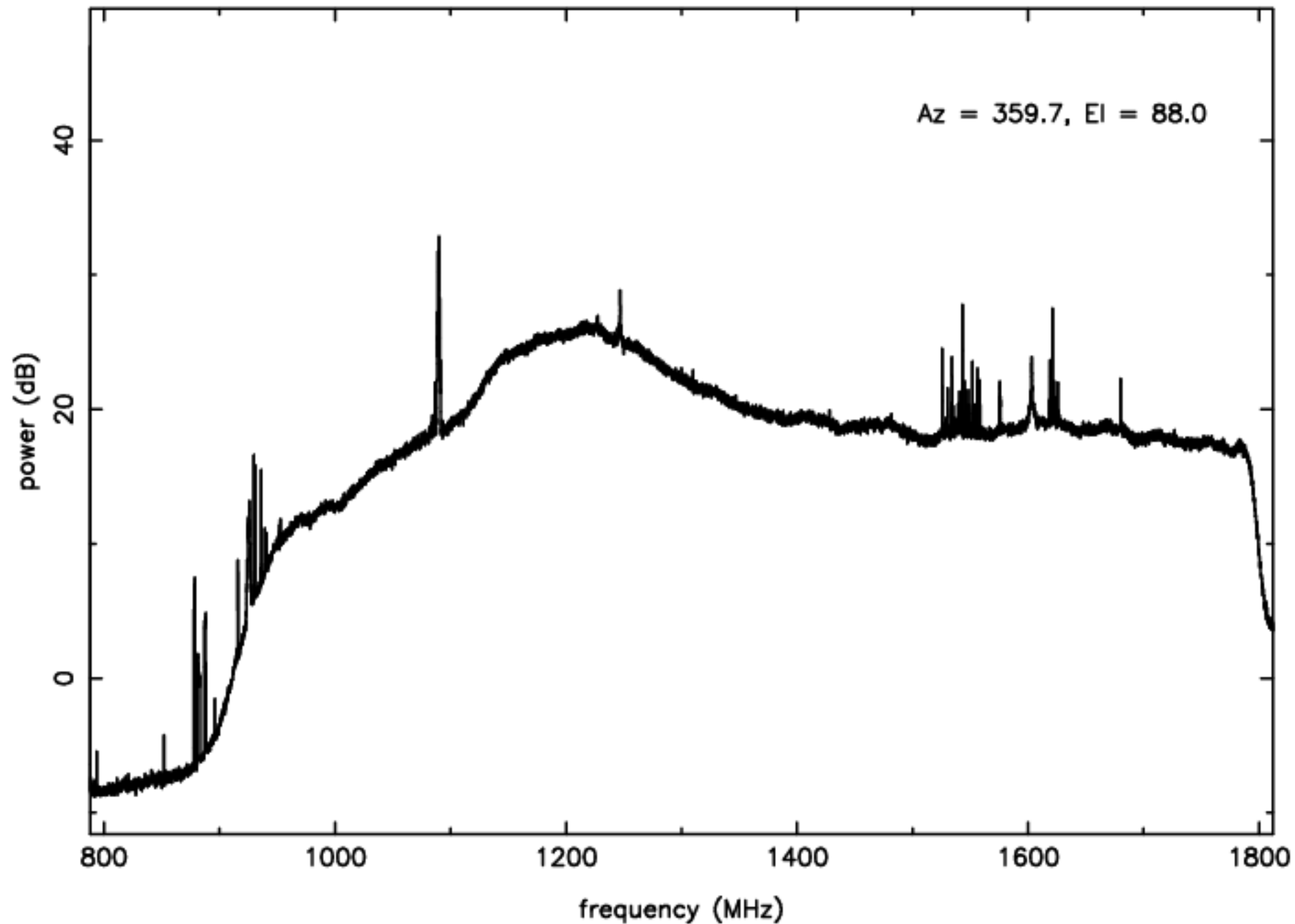
L-band RFI plot (mean power) – IF D – ea10
