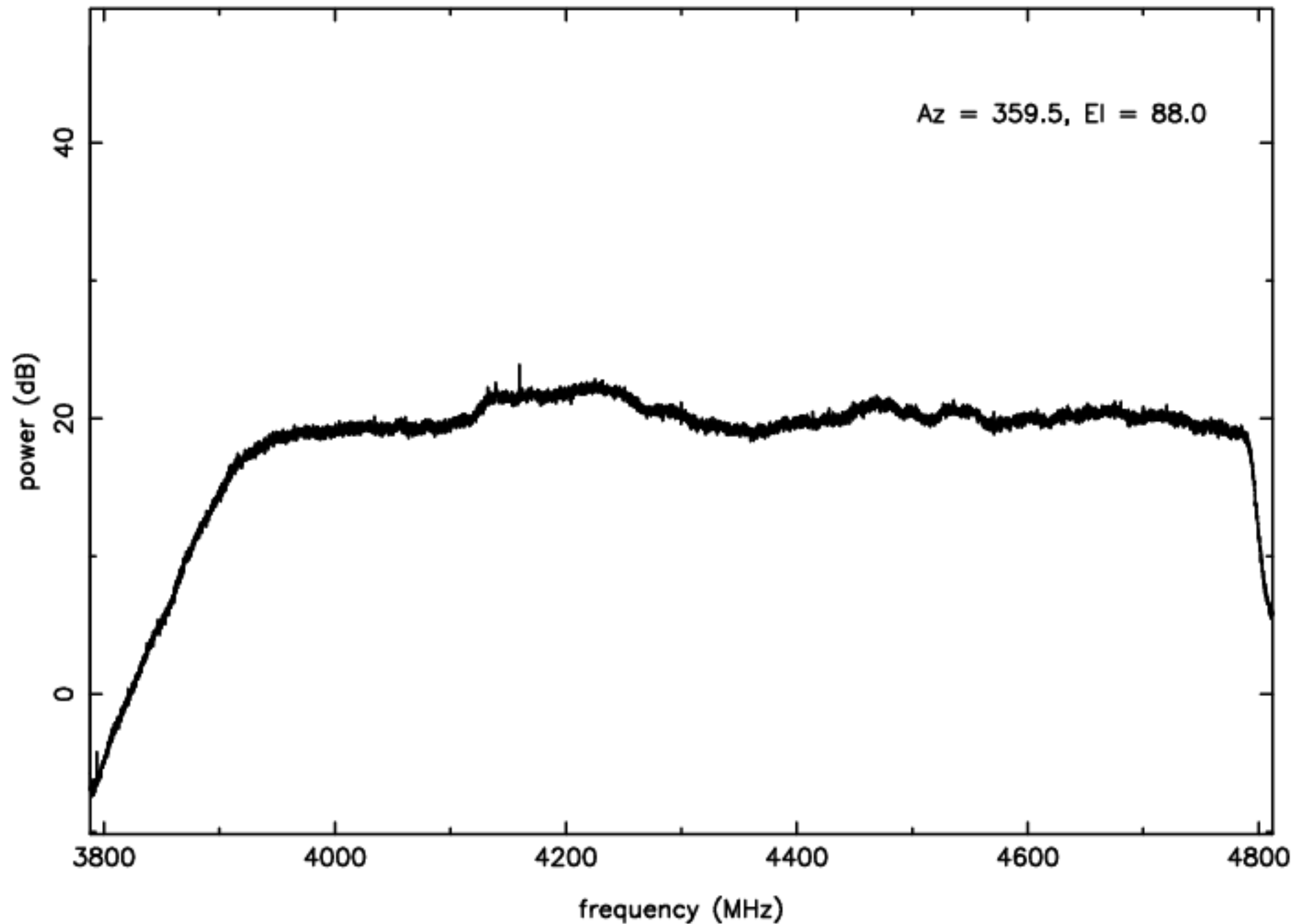
C-band RFI plot (mean power) – IF D – ea10
