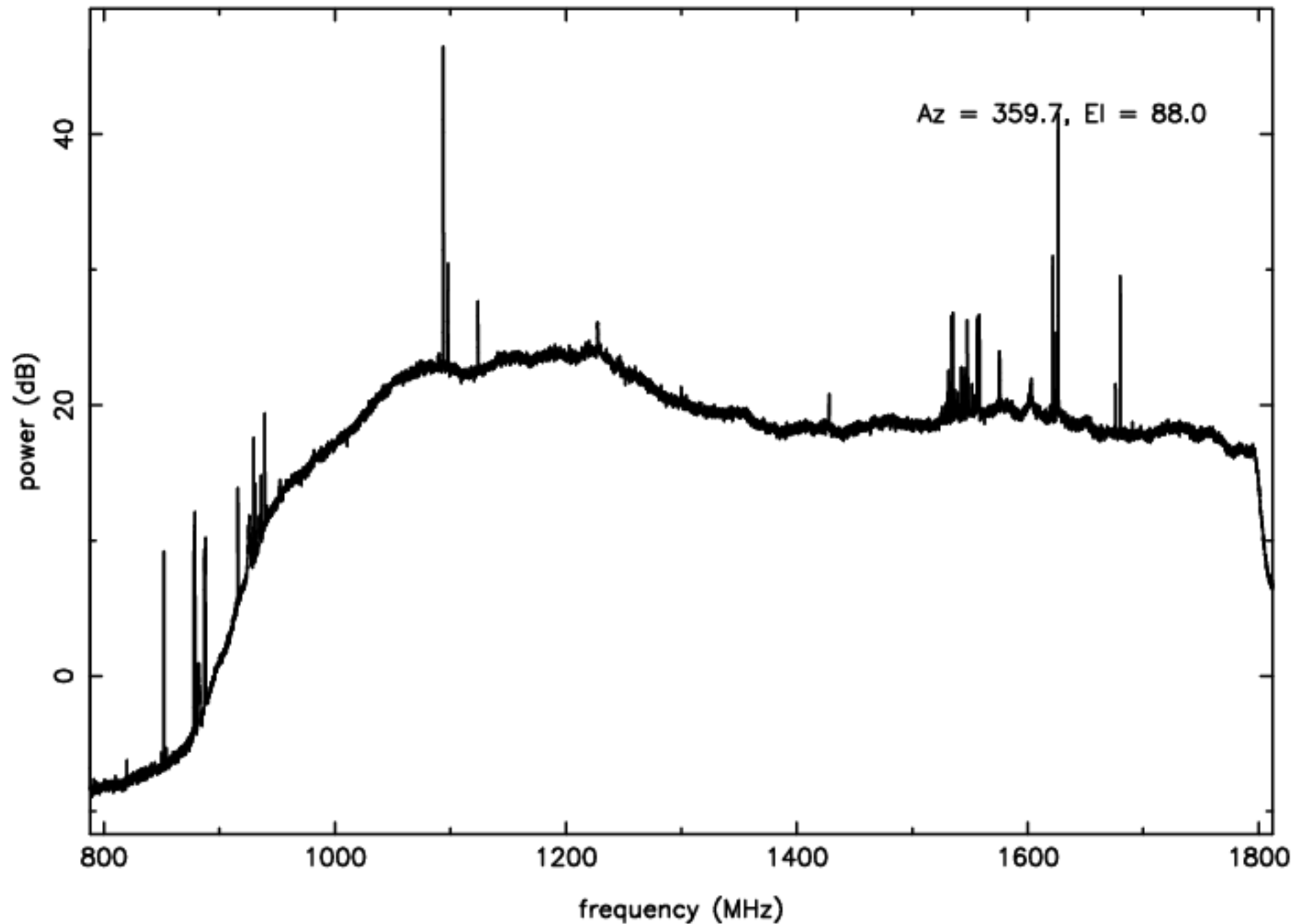
L-band RFI plot (mean power) – IF B – ea10
