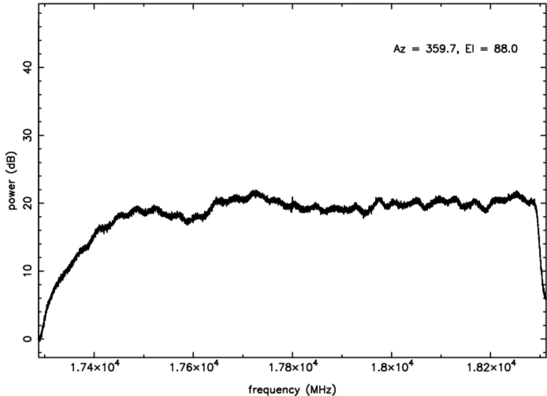
Ku-band RFI plot (mean power) – IF D – ea10
