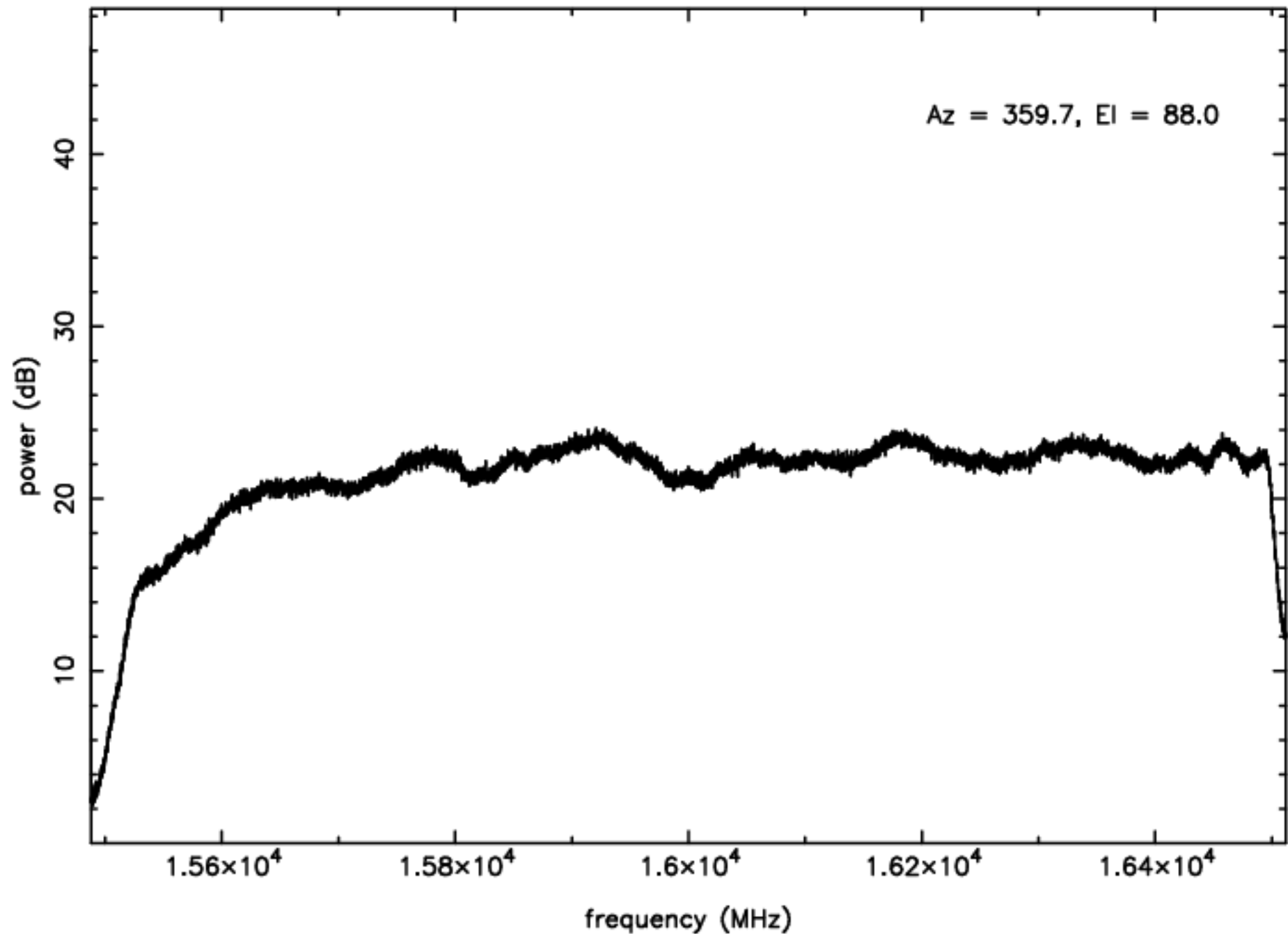
Ku-band RFI plot (mean power) – IF B – ea10
