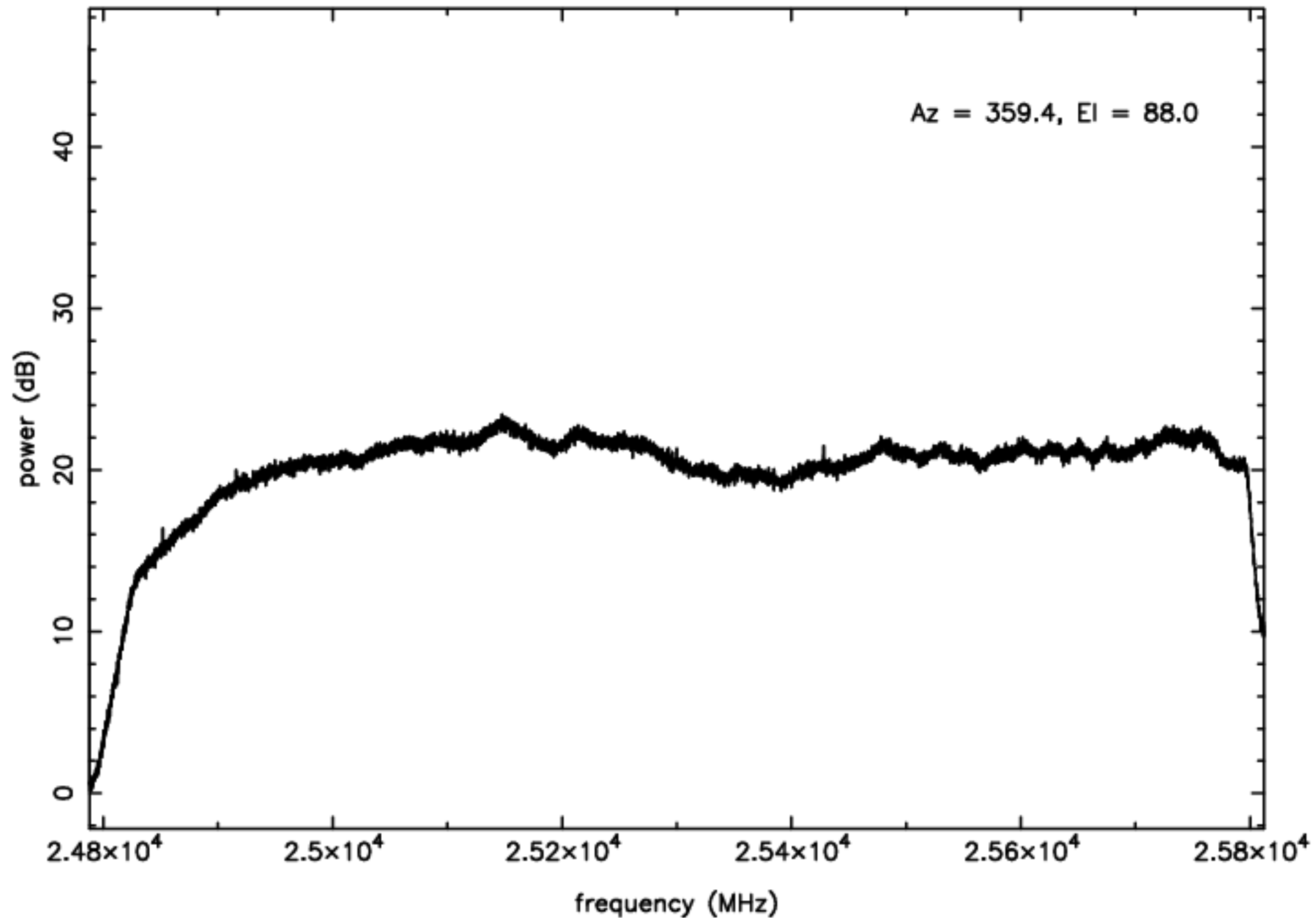
K-band RFI plot (mean power) – IF B – ea10
