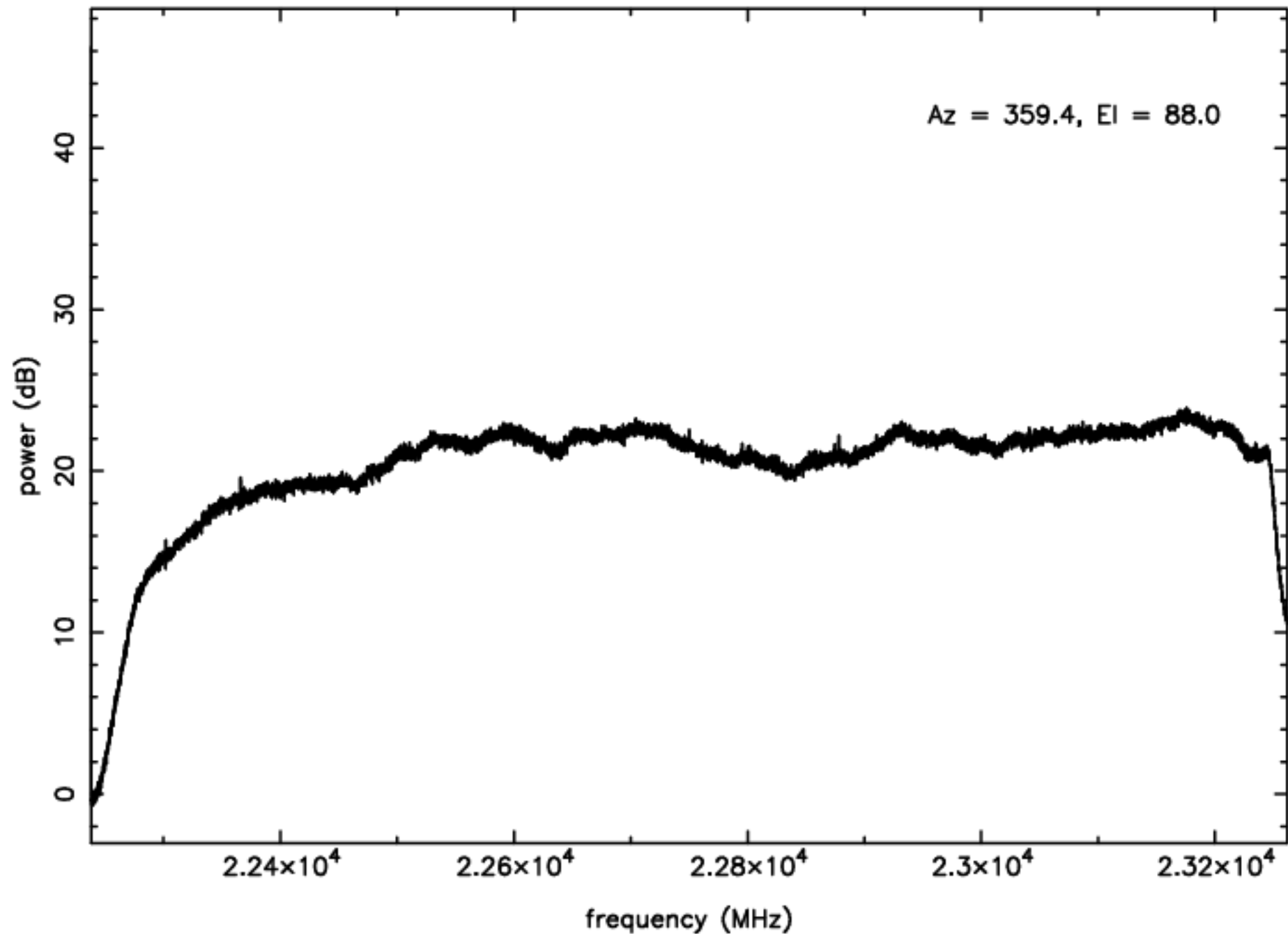
K-band RFI plot (mean power) – IF B – ea10
