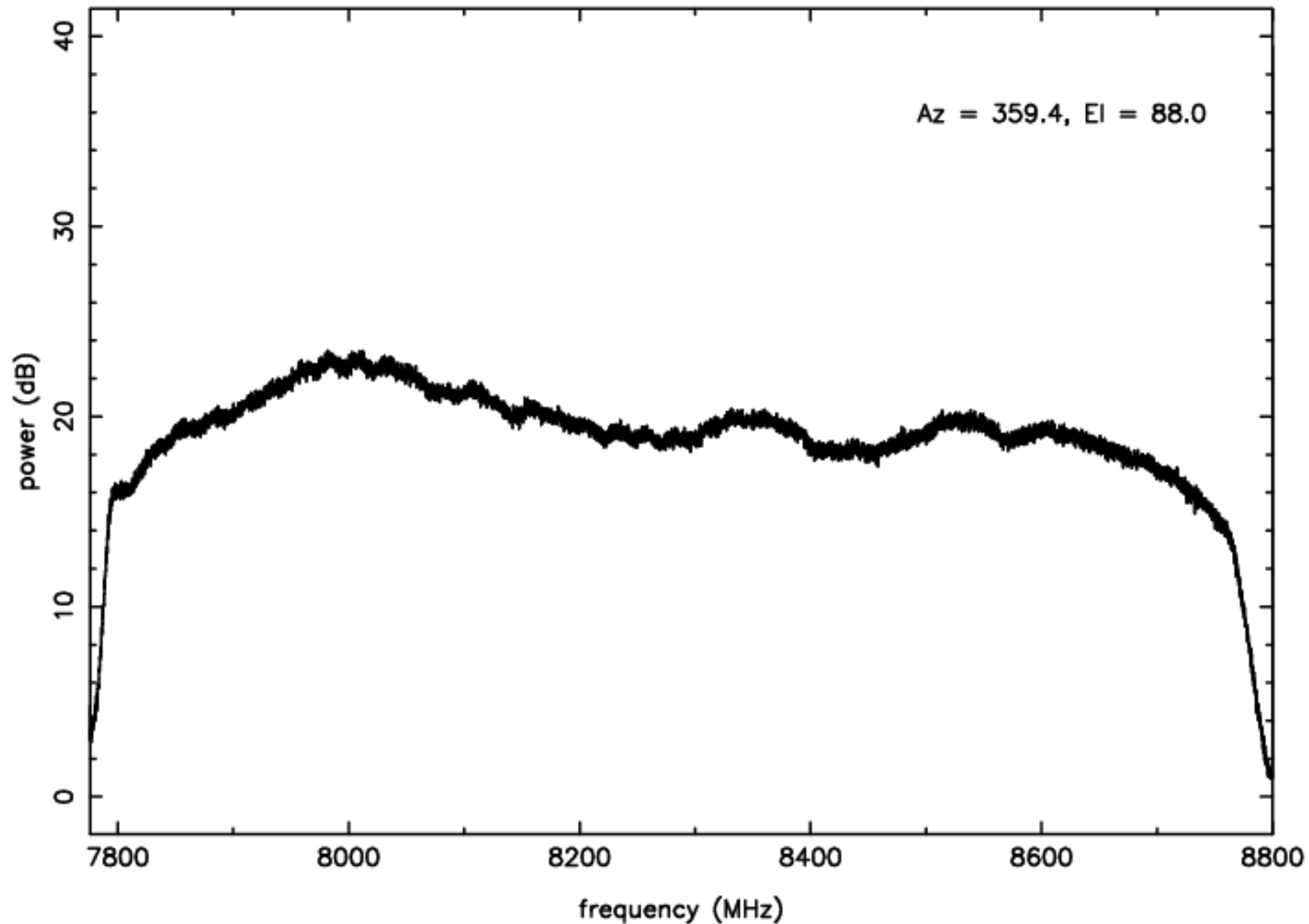
X-band RFI plot (mean power) – IF B – ea24
