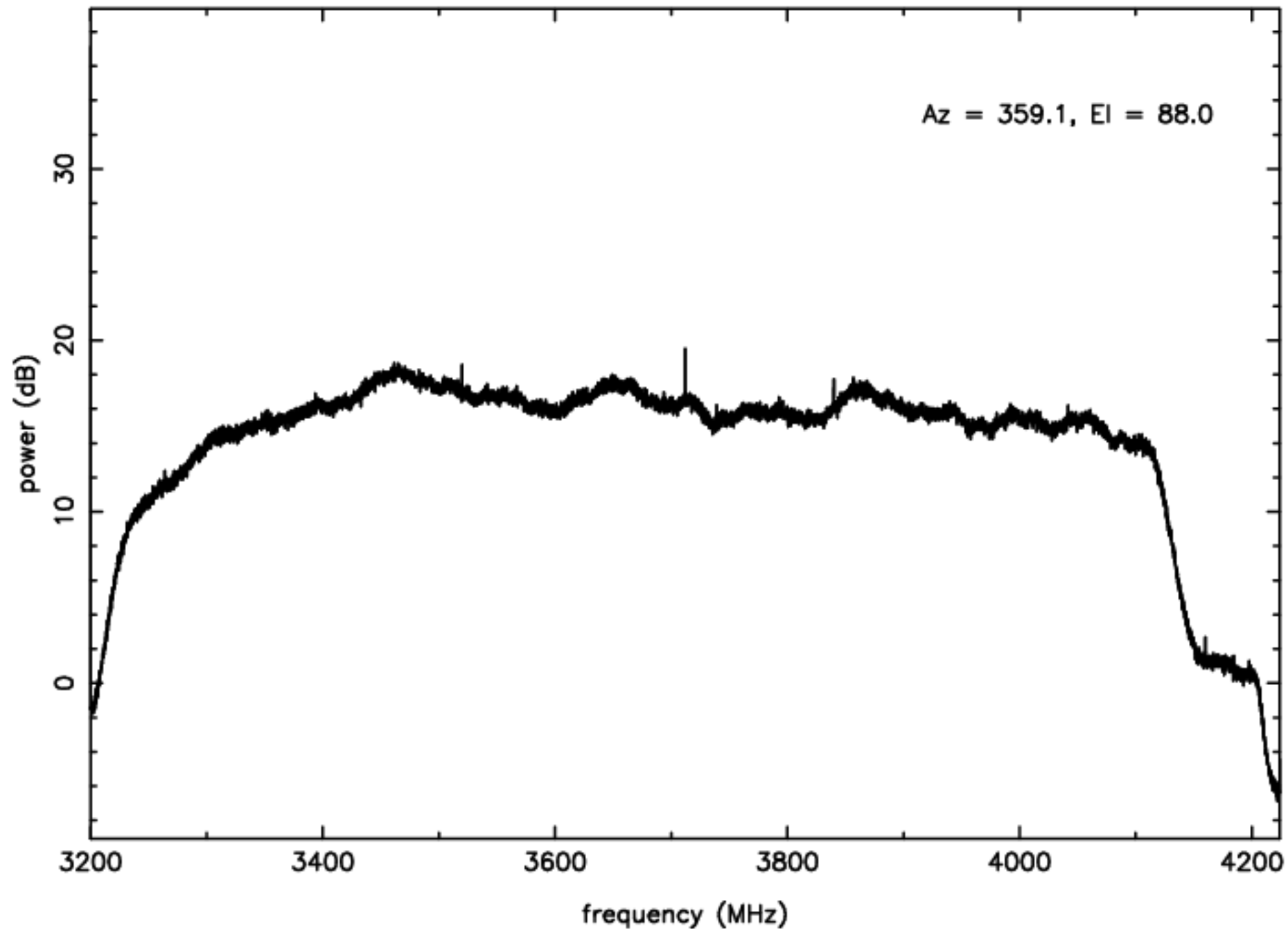
S-band RFI plot (mean power) – IF D – ea24
