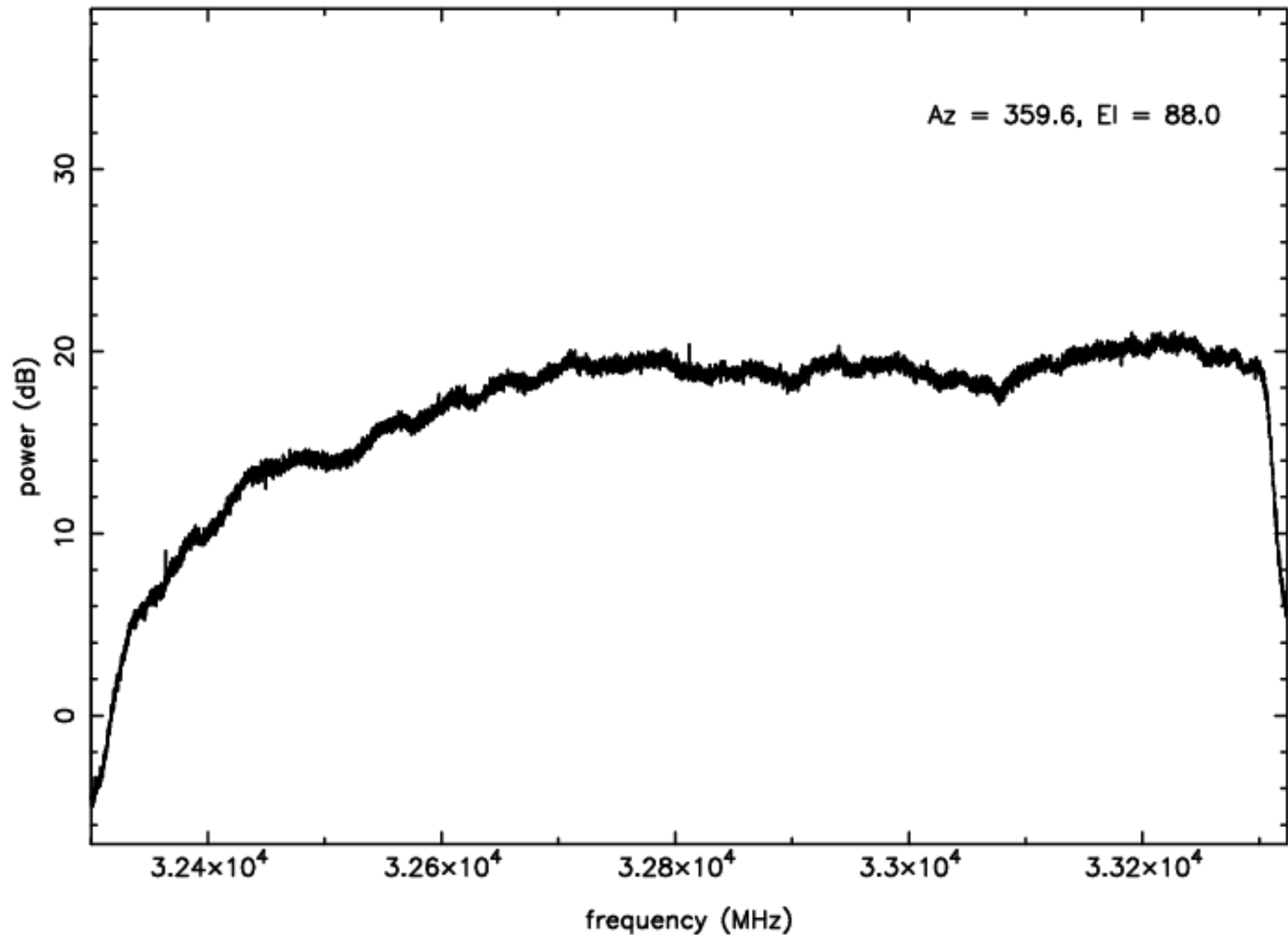
Ka-band RFI plot (mean power) – IF D – ea24
