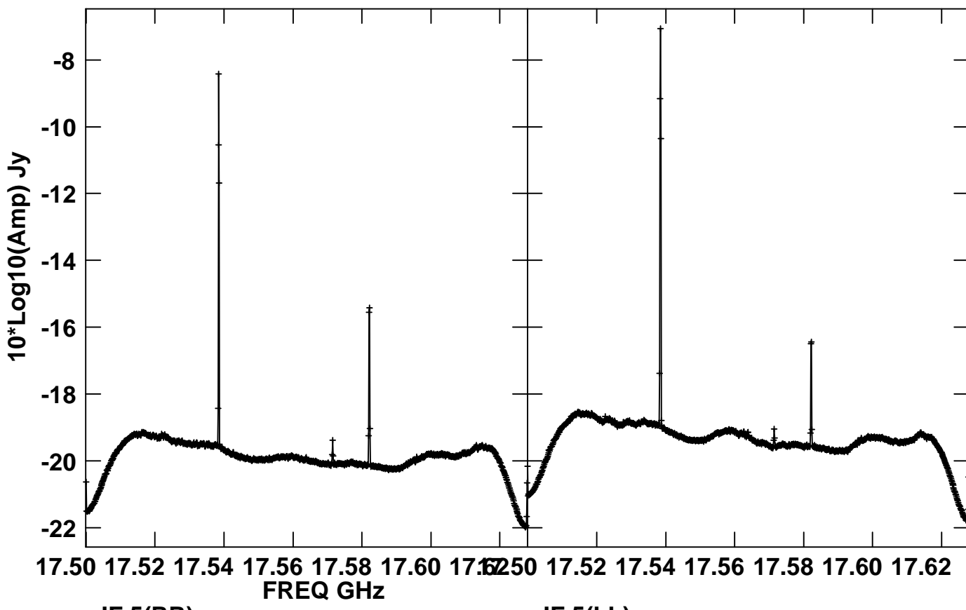
IF 5(RR) IF 5(LL) Scalar averaged cross-power spectrum Several baselines averaged
