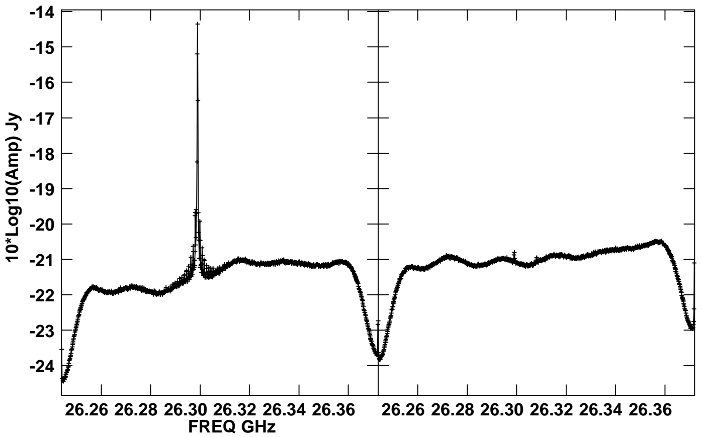
IF 3(RR) IF 3(LL) Scalar averaged cross-power spectrum Several baselines averaged
