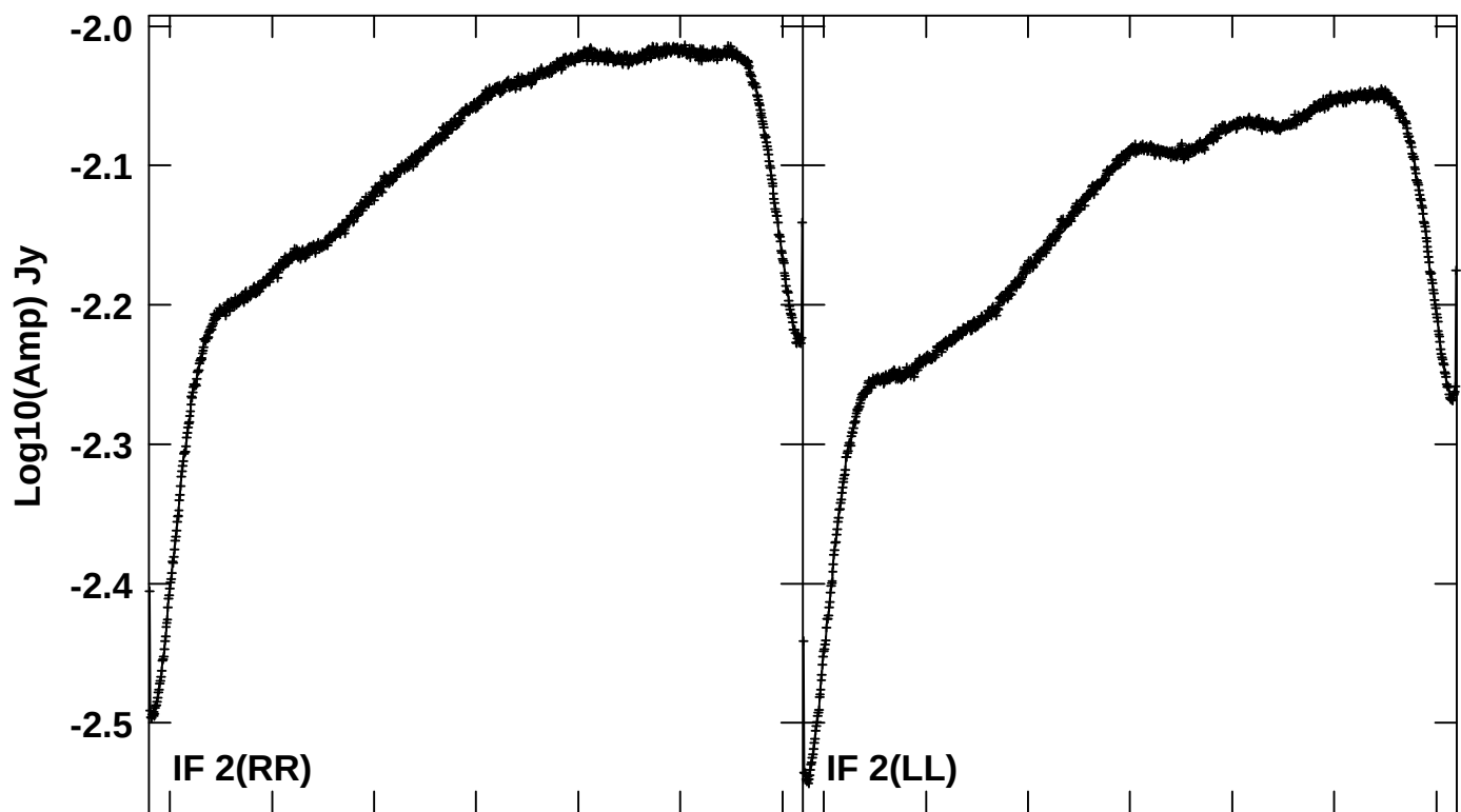
45120 45140 45160 45180 45200 45220 45240 45210 FREQ MHz Scalar averaged cross-power spectrum Several baselines averaged
