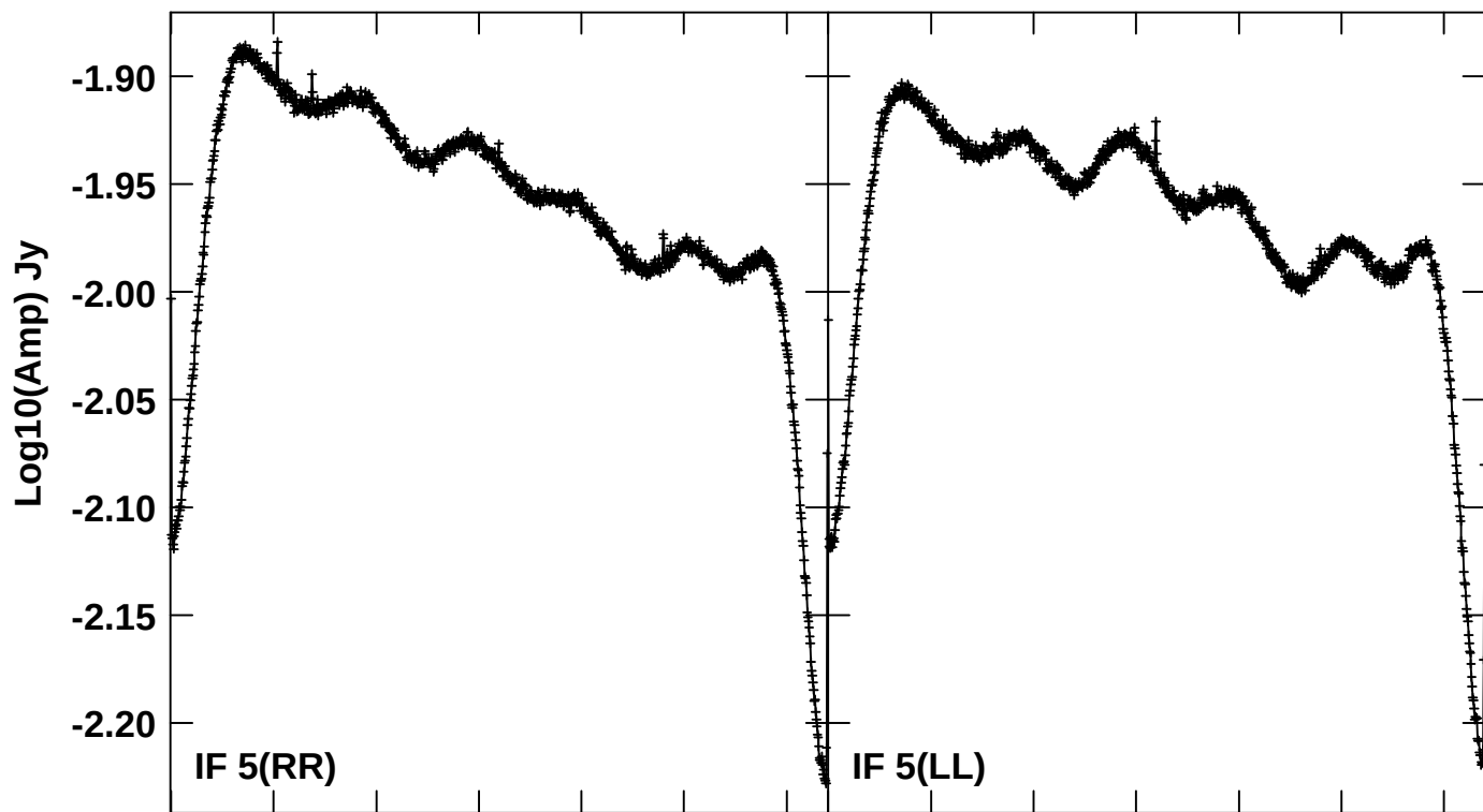
40500 40520 40540 40560 40580 40600 40620 FREQ MHz Scalar averaged cross-power spectrum Several baselines averaged
