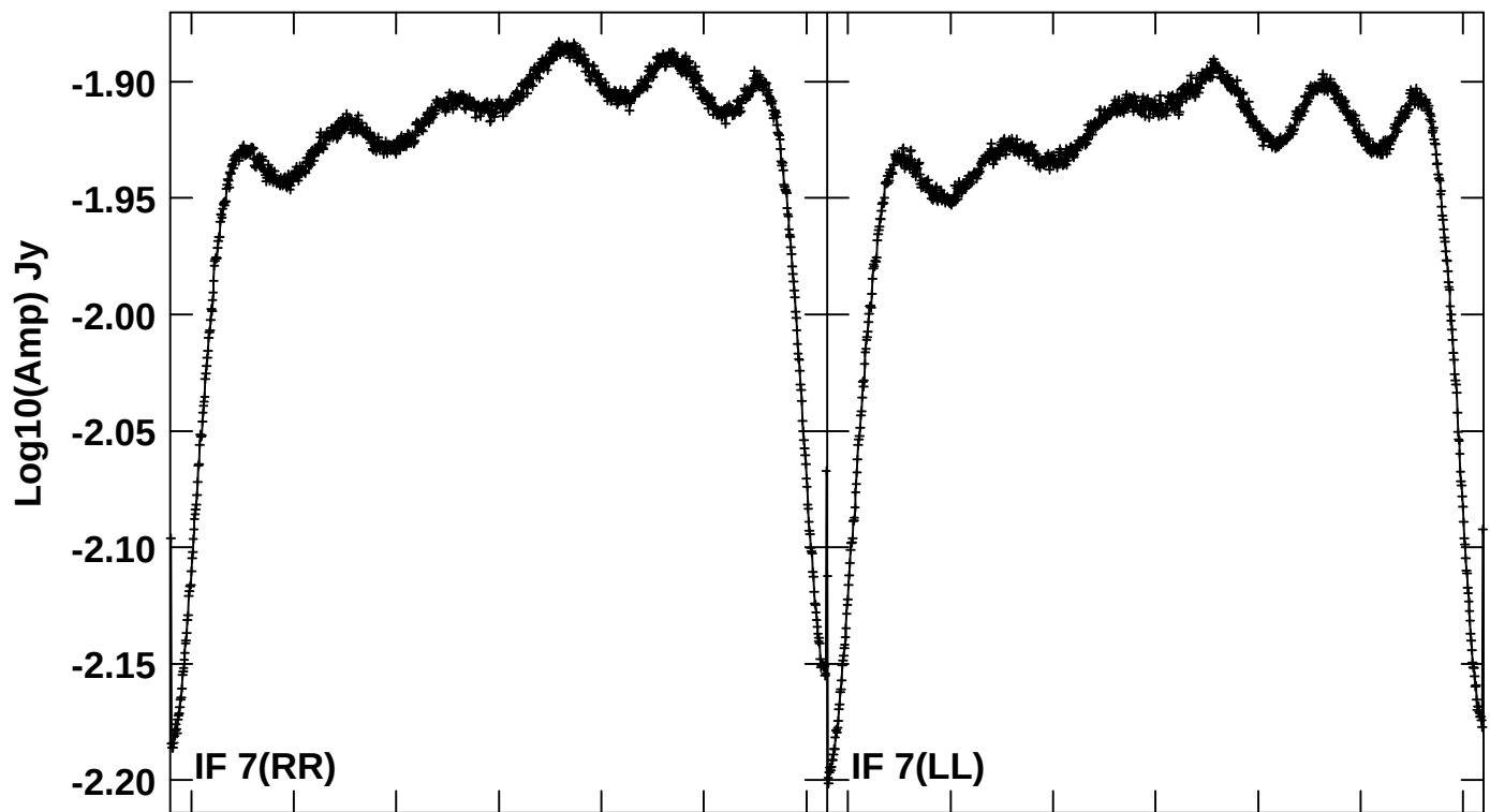
45760 45780 45800 45820 45840 45860 45880 FREQ MHz Scalar averaged cross-power spectrum Several baselines averaged
