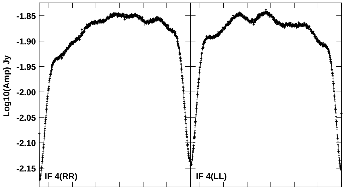
49380494004942049440494604948049500 FREQ MHz Scalar averaged cross-power spectrum Several baselines averaged
