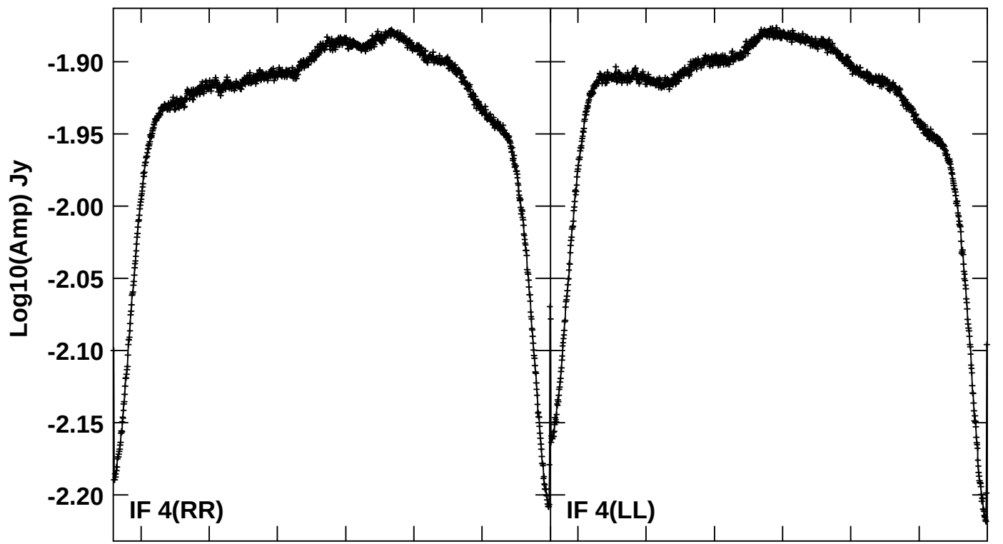
42380 42400 42420 42440 42460 42480 42500 42500 42480 42460 42440 42420 42400 42380 FREQ MHz Scalar averaged cross-power spectrum Several baselines averaged
