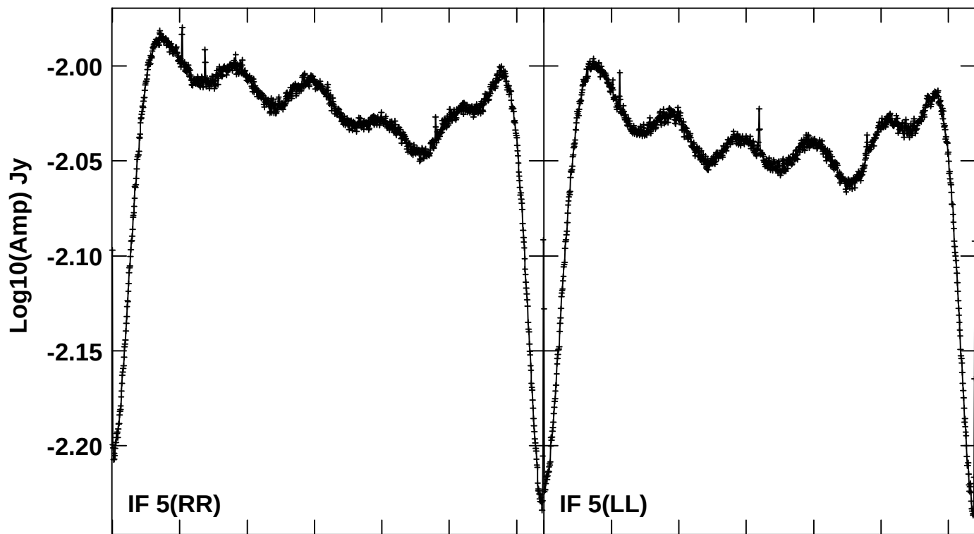
24500 24520 24540 24560 24580 24600 24620 FREQ MHz Scalar averaged cross-power spectrum Several baselines averaged
