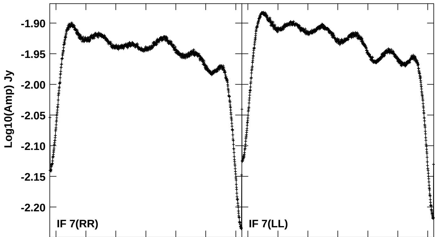
21760 21780 21800 21820 21840 21860 21880 FREQ MHz Scalar averaged cross-power spectrum Several baselines averaged
